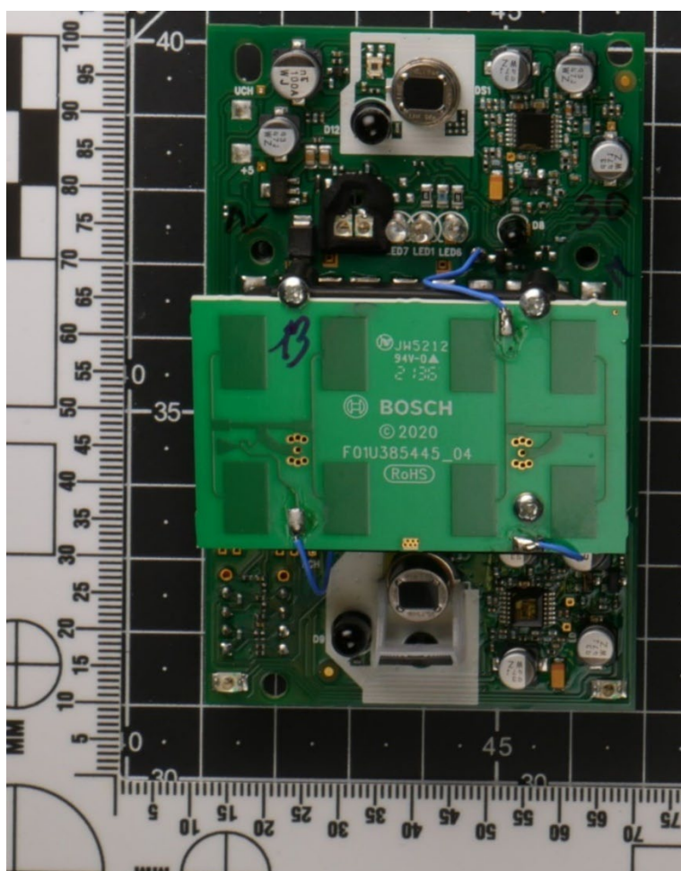
Main PCB & Microwave PCB TOP View
