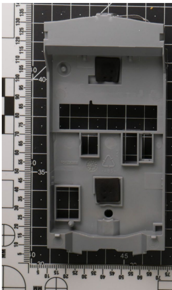
Inside Carrier w/PCBs removed
