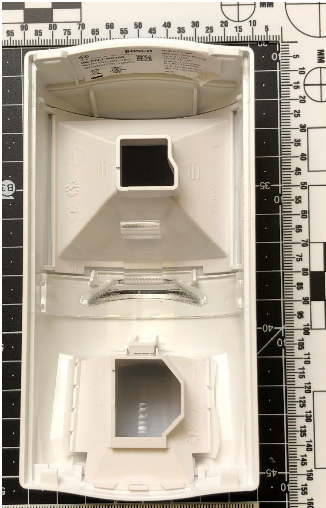
INSIDE FRONT COVER w/PCB & PCB Carrier removed
