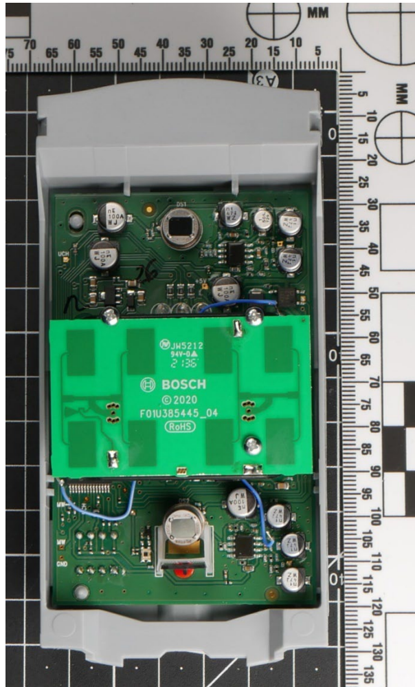
PCBs Main & Microwave in Carrier
