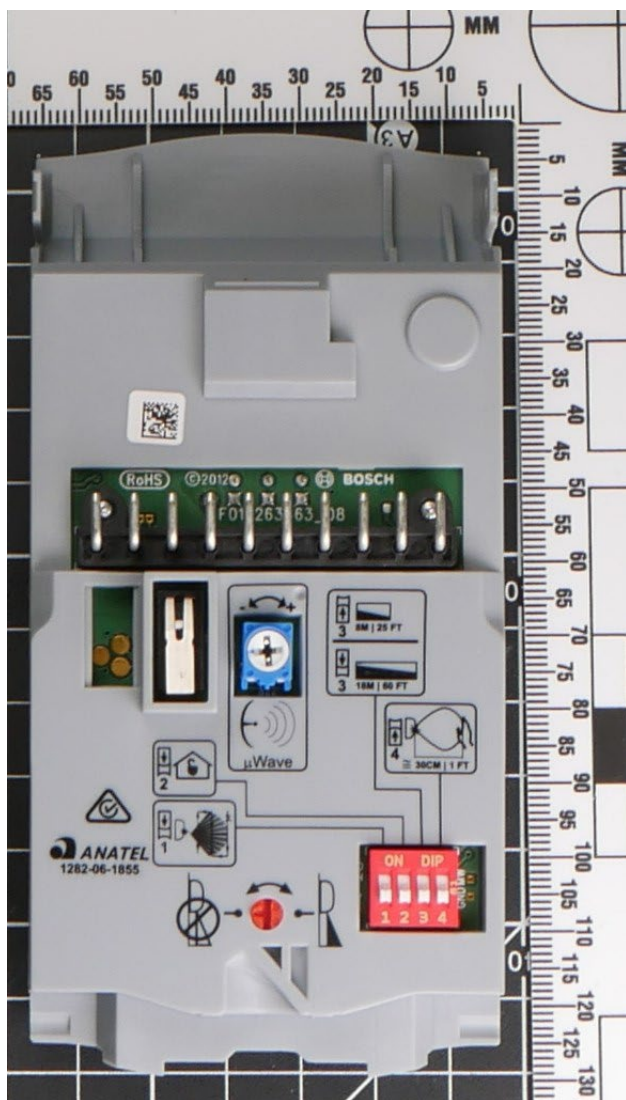
INSIDE FRONT w/Back Cover Removed
