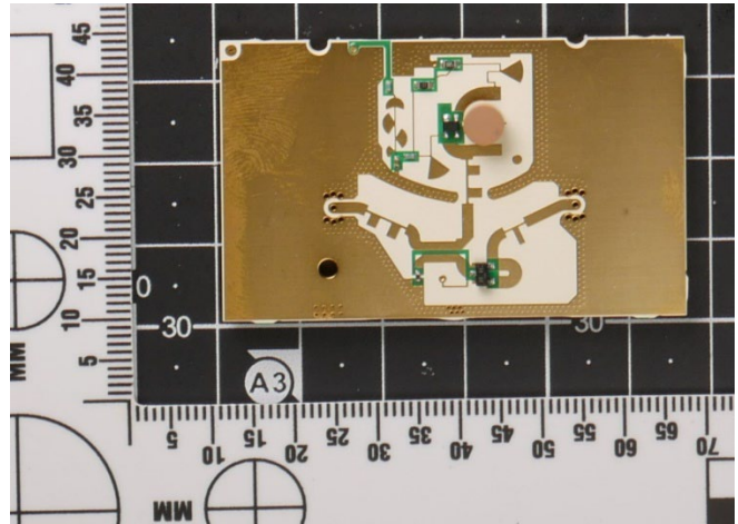
Microwave PCB Back w/o BackShield
