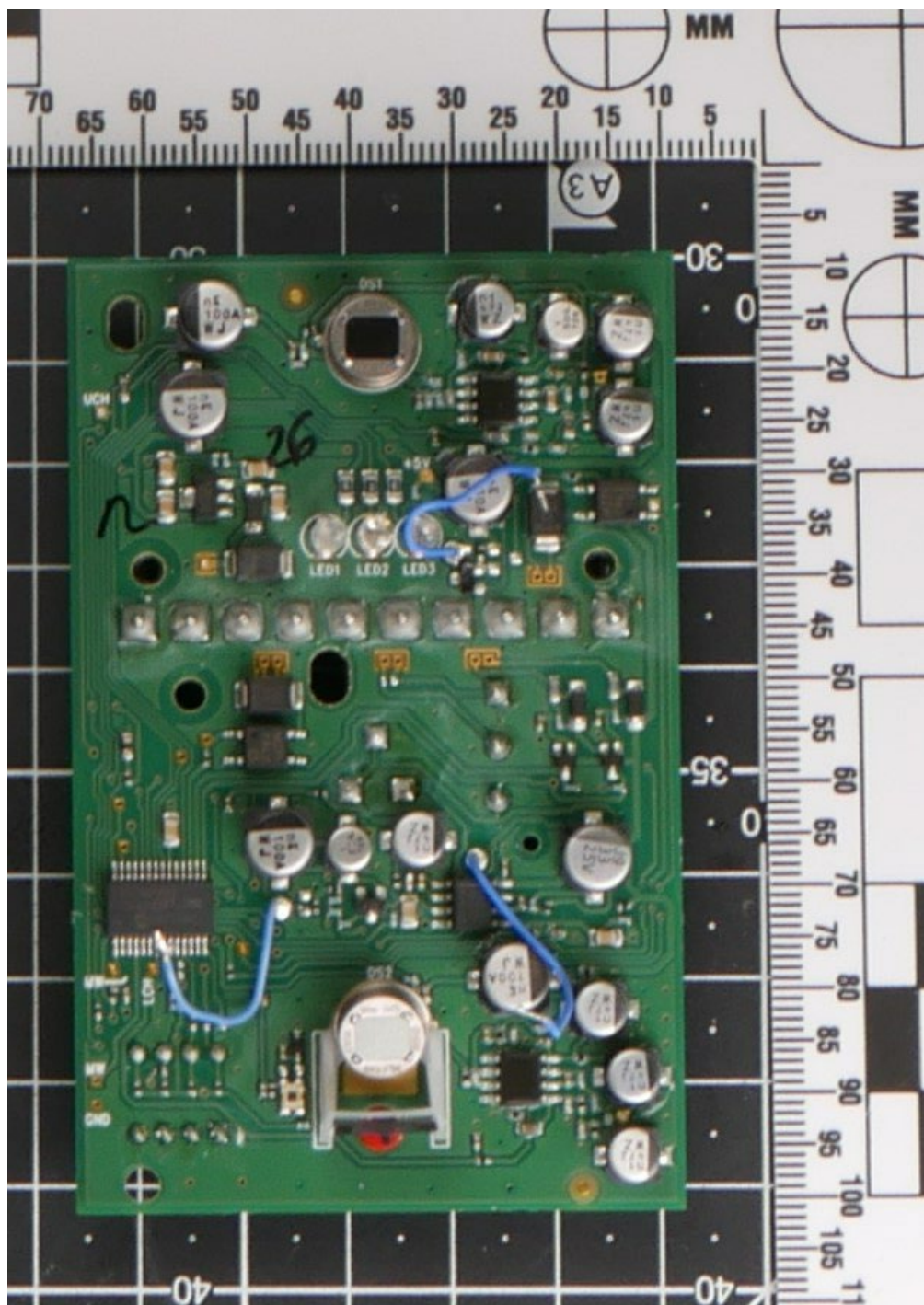
Main PCB TOP w/Microwave PCB removed
