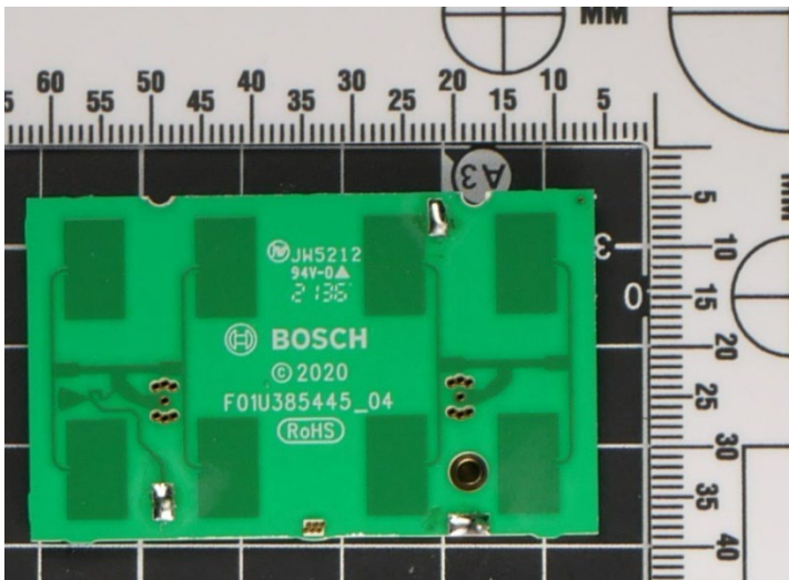
Microwave PCB Top
