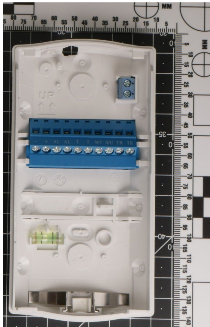
INSIDE BACK COVER
