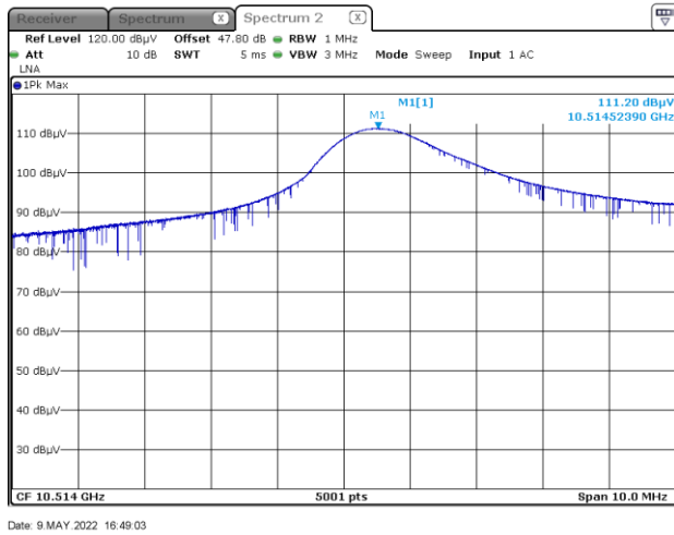
Figure 8.5-7: Field strength of fundamental emission – Mid Fundamental Frequency
