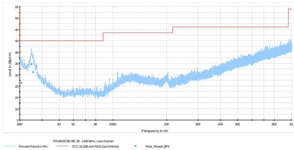
Figure 8.5-14: Field strength of spurious emissions 30–1000 MHz – Low Fundamental Frequency
