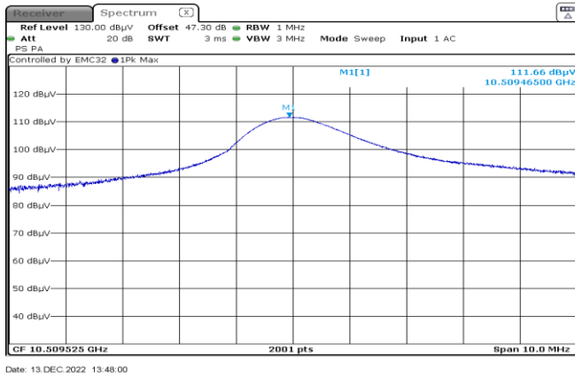
Figure 8.5-1: Field strength of fundamental emission – Low Fundamental Frequency
