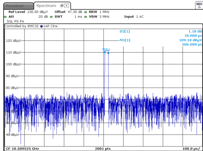
Figure 8.5-13: Pulse width
