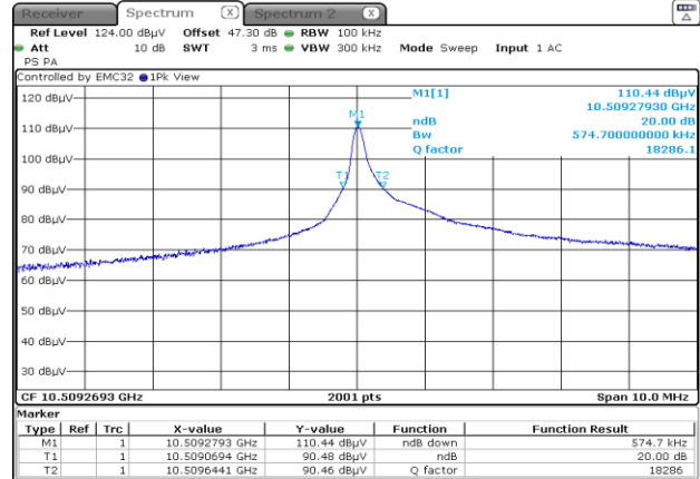
Figure 8.6-2: 20 dB occupied bandwidth – Low Fundamental Frequency
