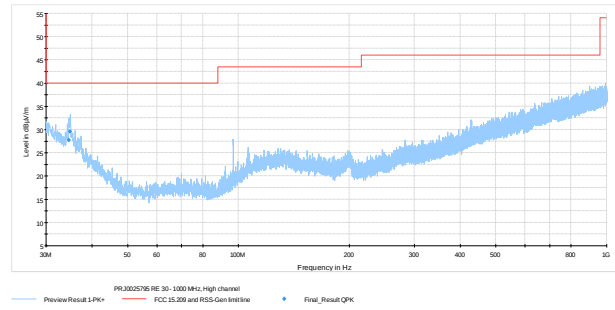
Figure 8.5-15: Field strength of spurious emissions 30–1000 MHz – High Fundamental Frequency
