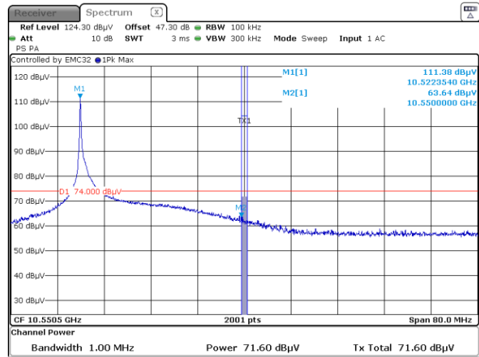
Figure 8.5-11: Field strength of upper bandedge emission
