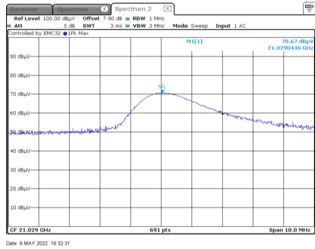
Figure 8.5-8: Field strength of 2 nd harmonic emission – Mid Fundamental Frequency
