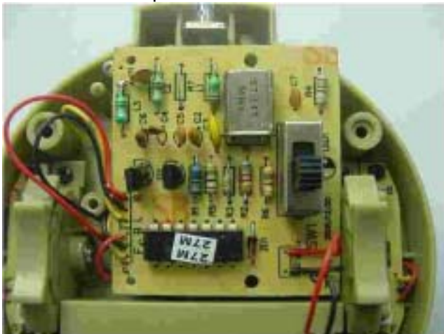
Component Side View
