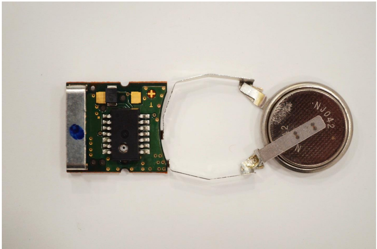
PWB Bottom
