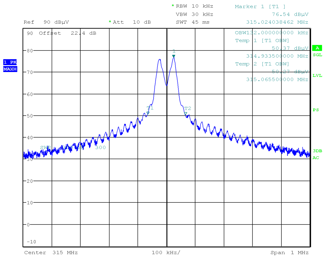
99% Occupied Bandwidth
