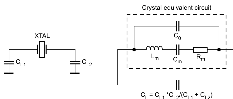
Figure 3-2. XTAL with Load Capacitance
