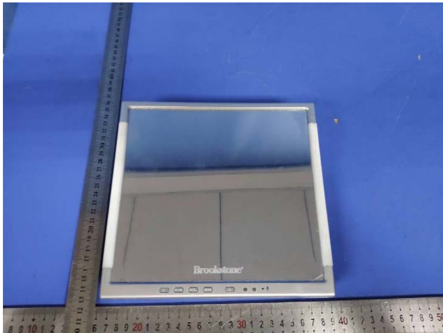
Test Model No. 1703
