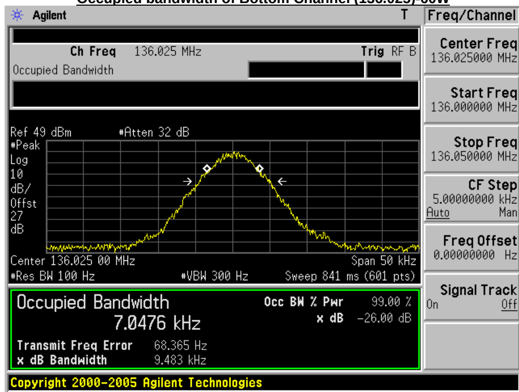
Occupied bandwidth of Bottom Channel (136.025)-60W
