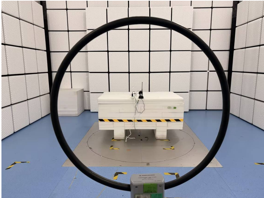
RE_9kHz~30MHz(Powered by Adapter)
