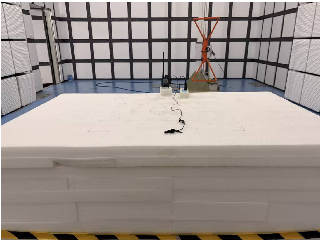
RE – Rear View _30MHz~1GHz (Powered by adapter)
