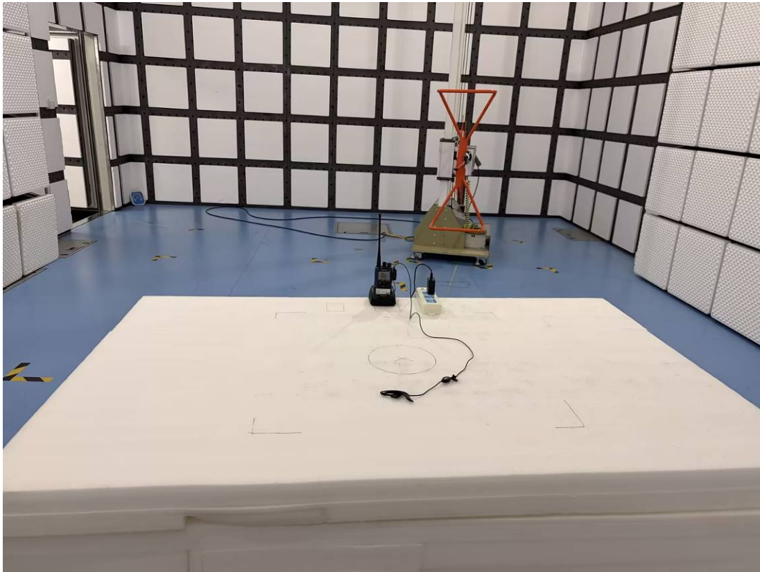
RE – Rear View _30MHz~1GHz (Powered by charger)
