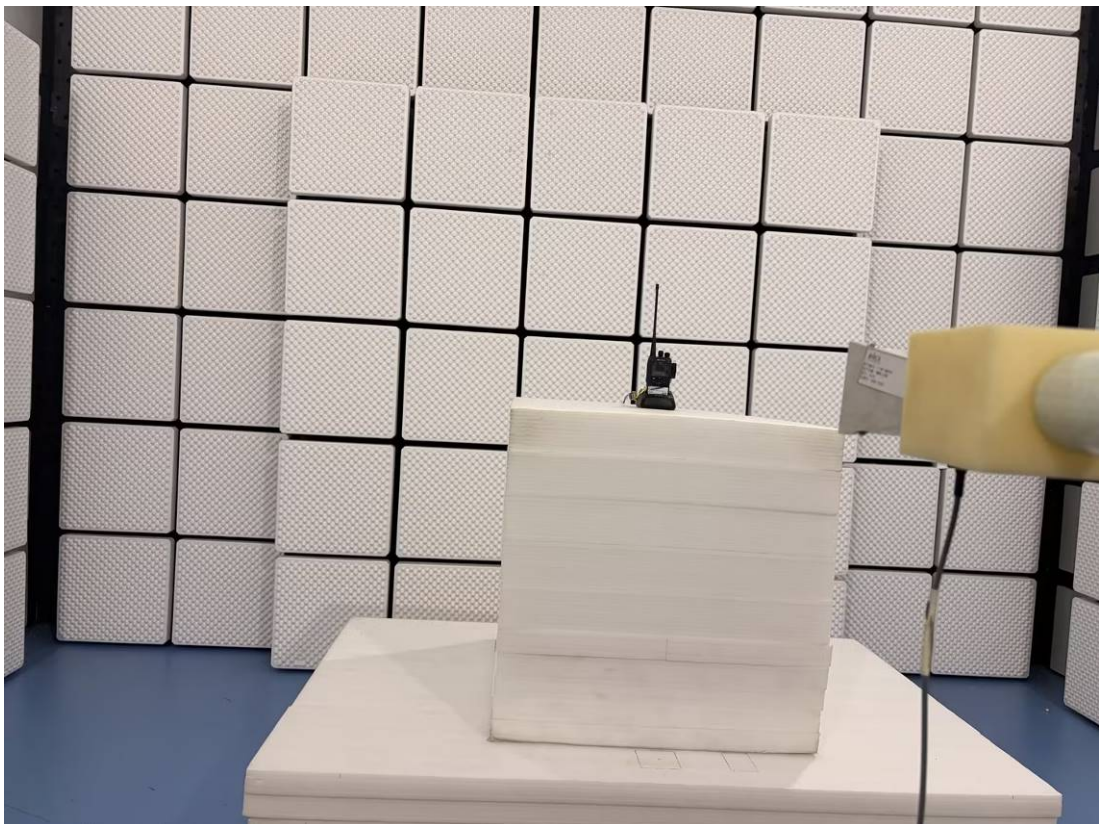
RE – Rear View (18 GHz~25 GHz)
