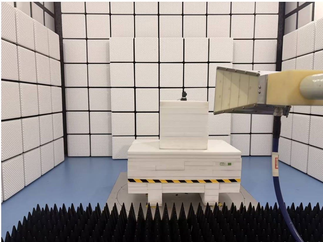
RE – Rear View (1 GHz~18 GHz)
