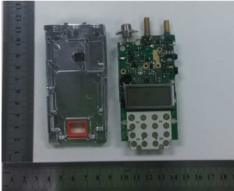
5. Mainboard front view without shielding
