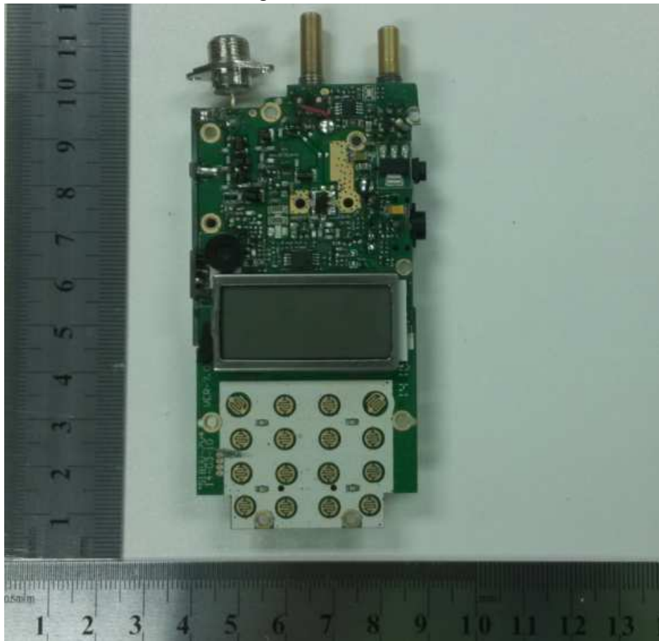
5. Mainboard front view without shielding
