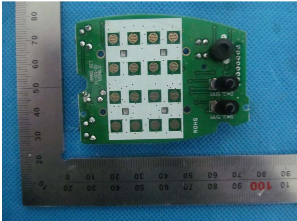
INTERNAL VIEW-9 OF EUT
