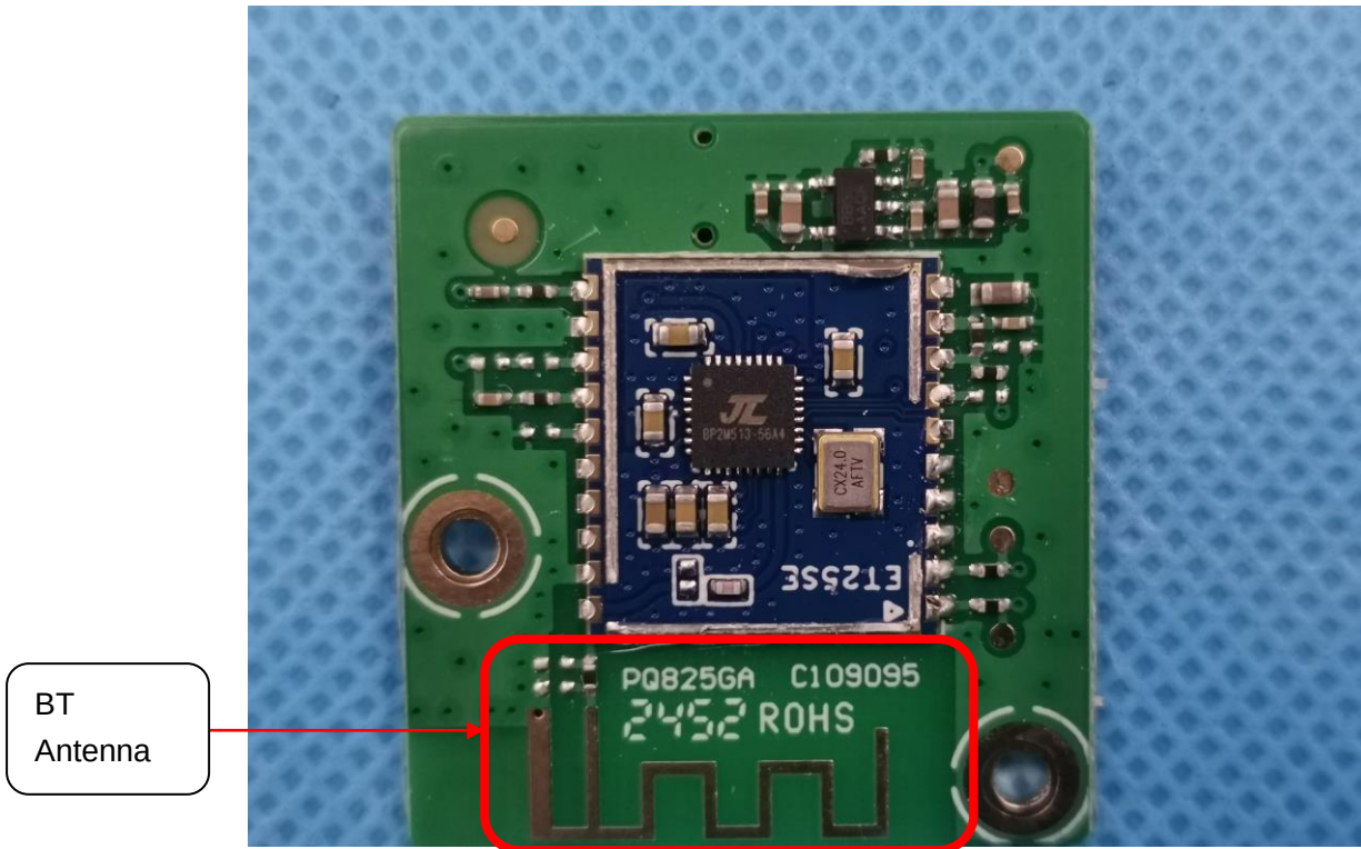
Internal View of EUT (Figure 10)
