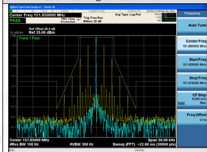
Emission Mask D@161.610MHz-0.2W-FM
