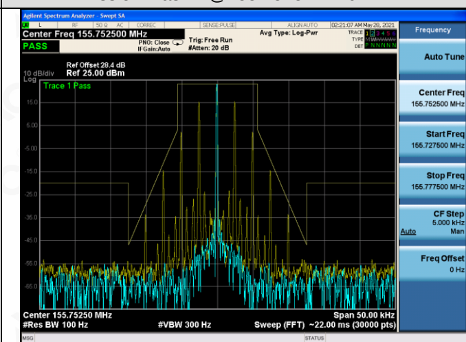
Emission Mask D@173.975MHz-0.2W-FM
