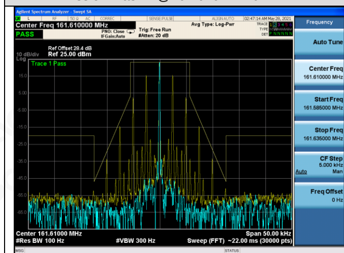
Emission Mask D@406.125MHz-6W-FM
