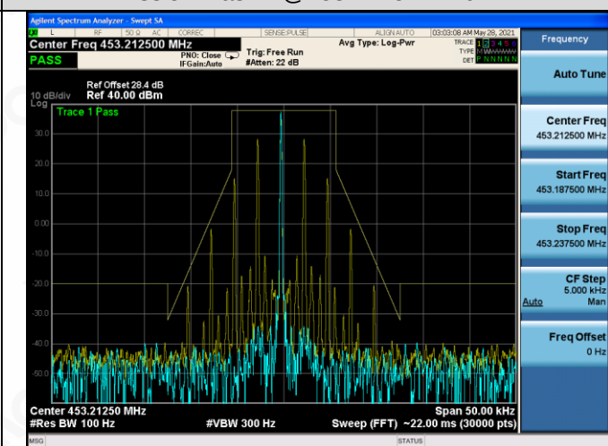
Emission Mask D@453.2125MHz-6W-FM
