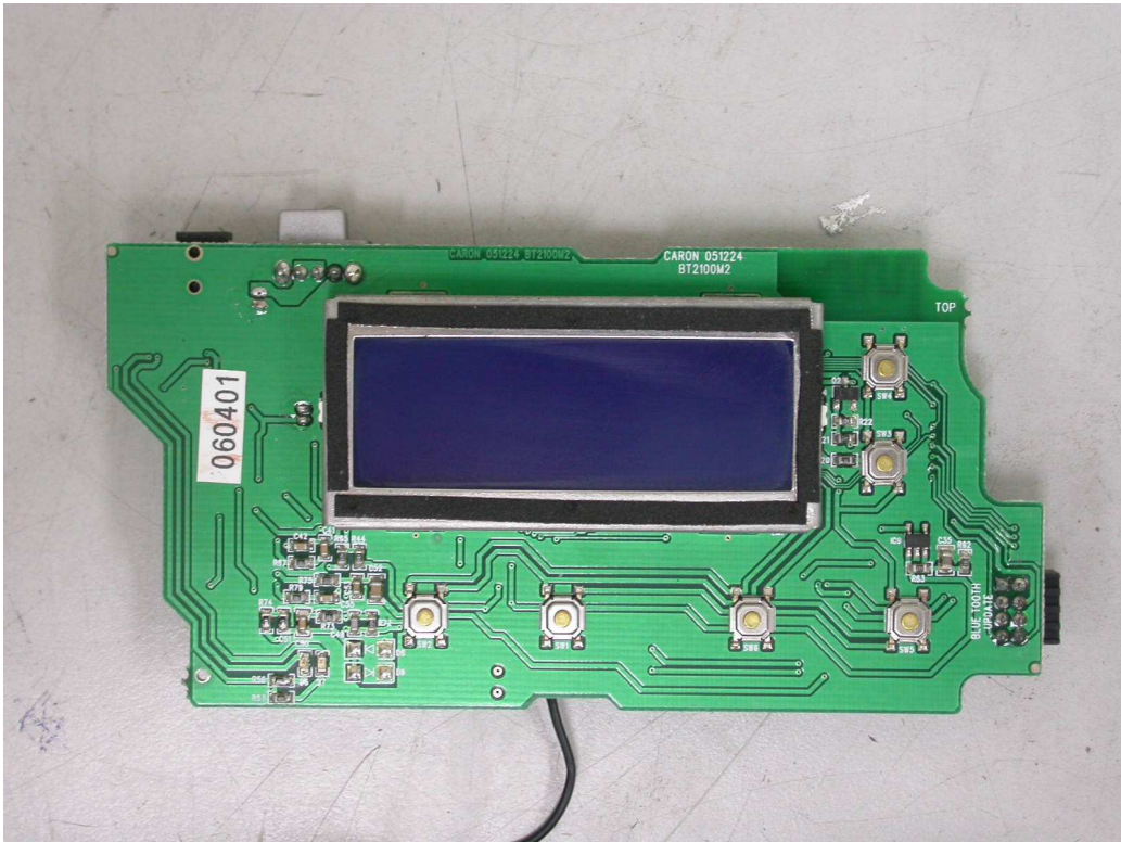
14. Front view of PCB
