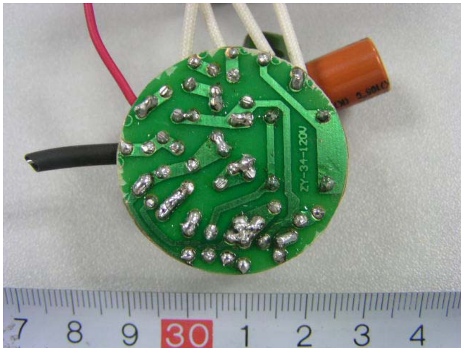
S-14W: EUT-PCB View (2)
