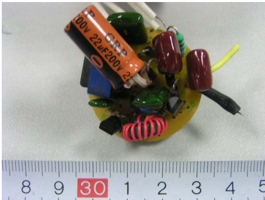
G-9W: EUT-PCB View (1)
