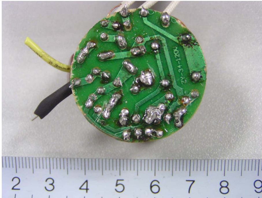
G-9W: EUT-PCB View (2)
