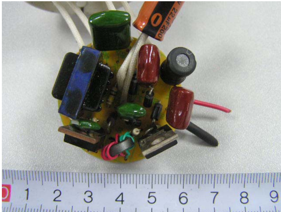
S-25W: EUT-PCB View (1)
