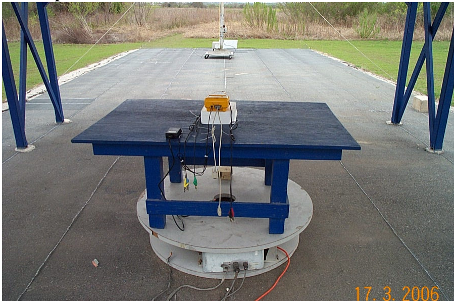
Figure 3, Spurious Radiated < 1 GHz, Rear
