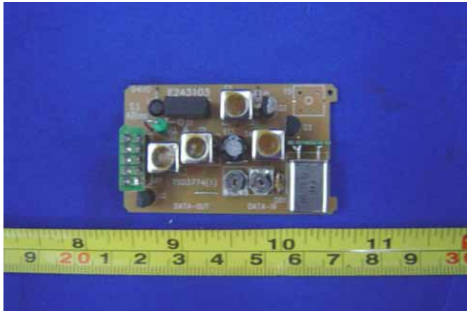
PCB(2) – Component View
