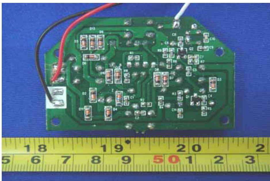
PCB (1) – Solder View
