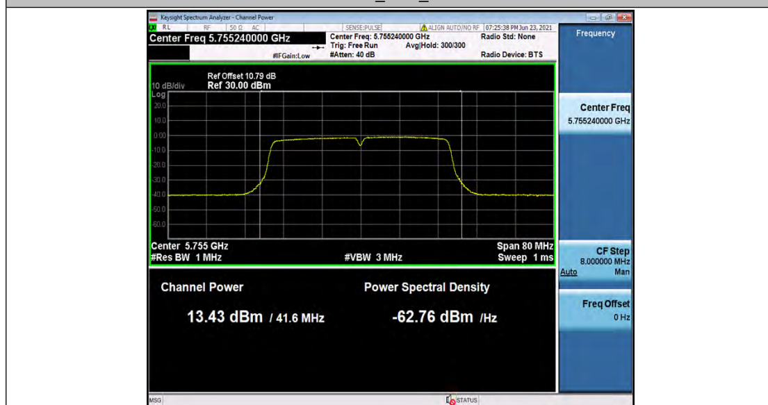
11AC40_Ant1_5755
