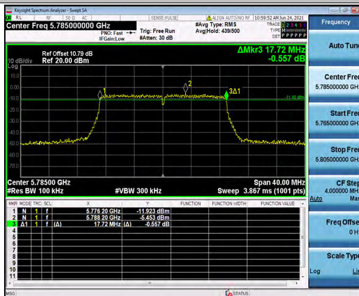
11AC20_Ant2_5785
