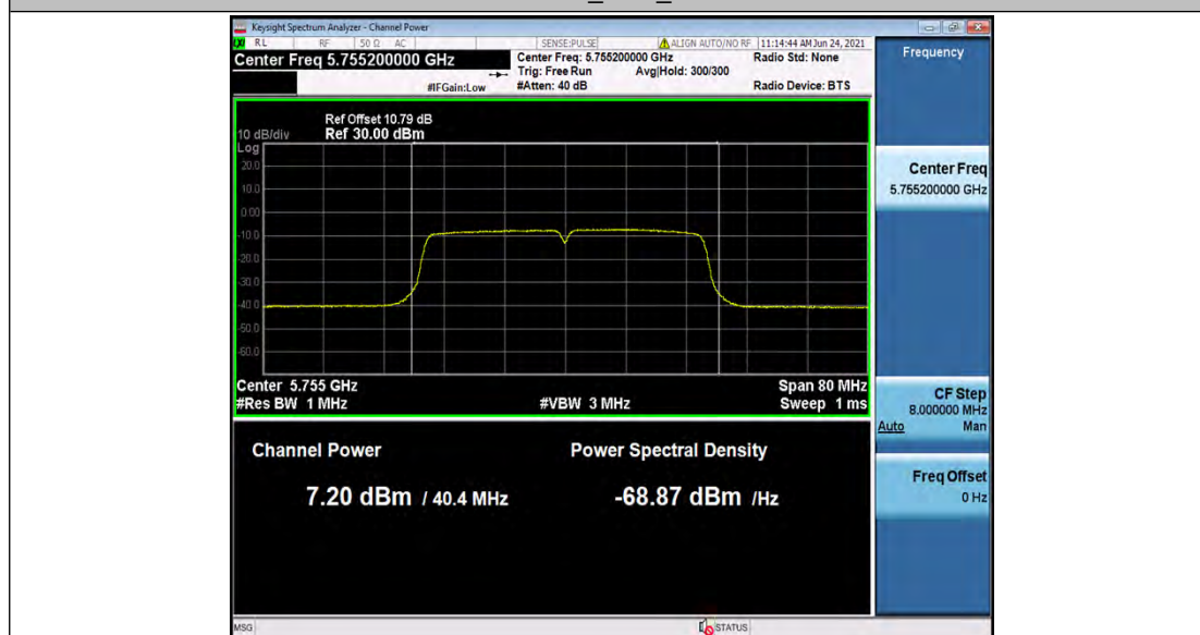
11AC40_Ant2_5755
