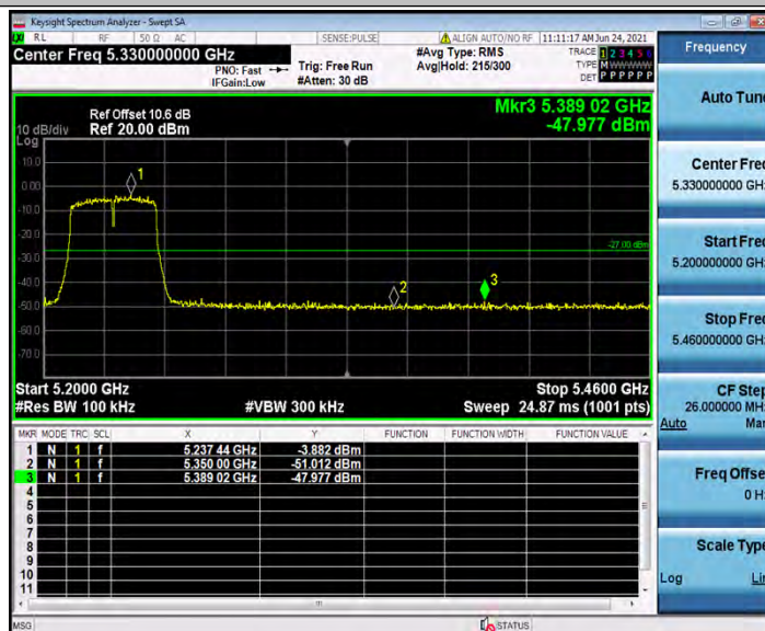
11AC40_Ant2_High_5230
