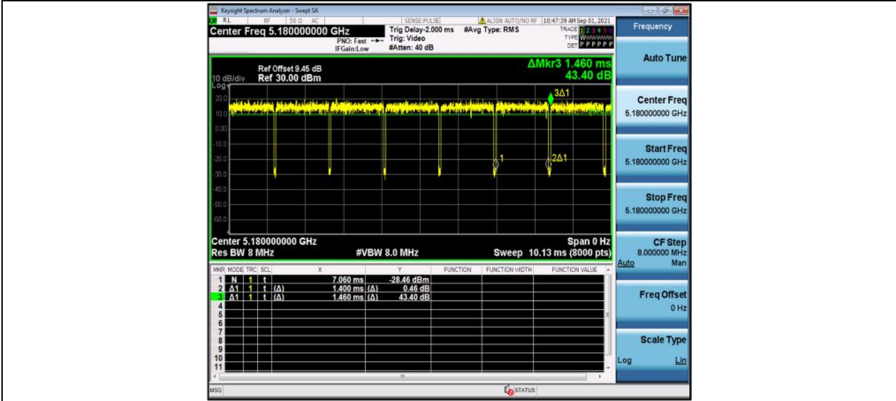
11A_Ant2_5180
