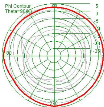
Gain(Peak):4.68dBi
