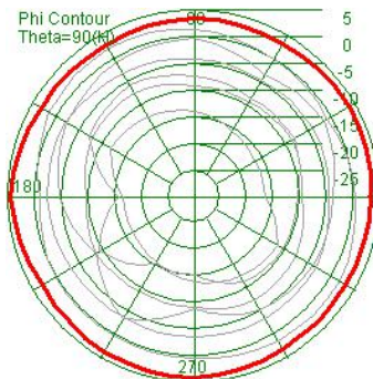
Gain(Peak):4.81dBi
