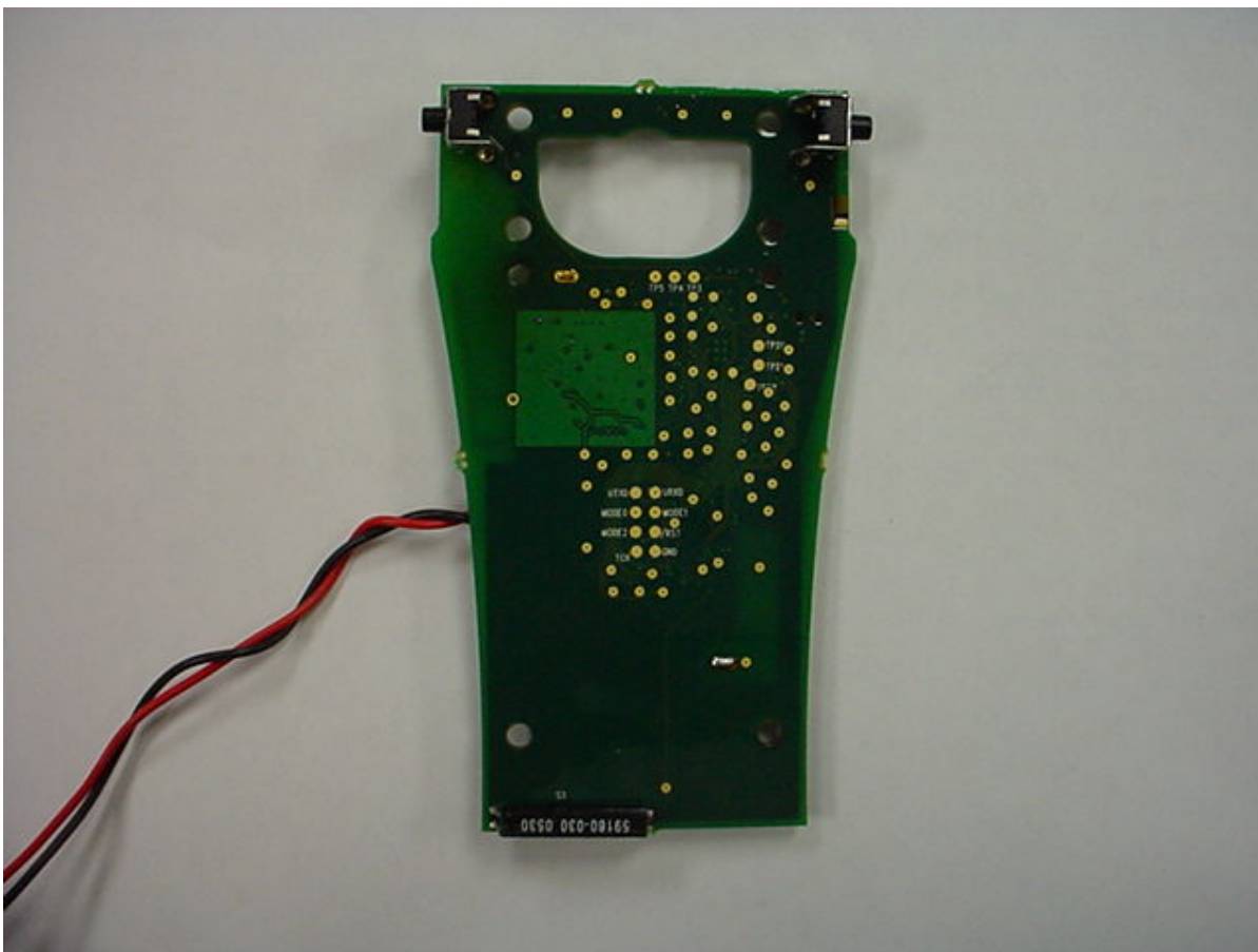
Photo Six – Internal PCB Side
