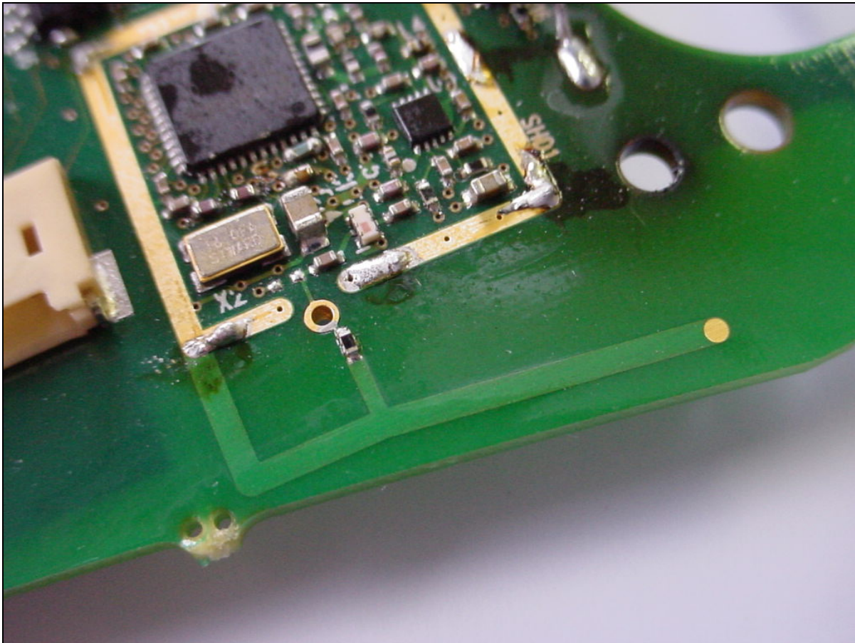
Photo Four – Internal PCB Antenna
