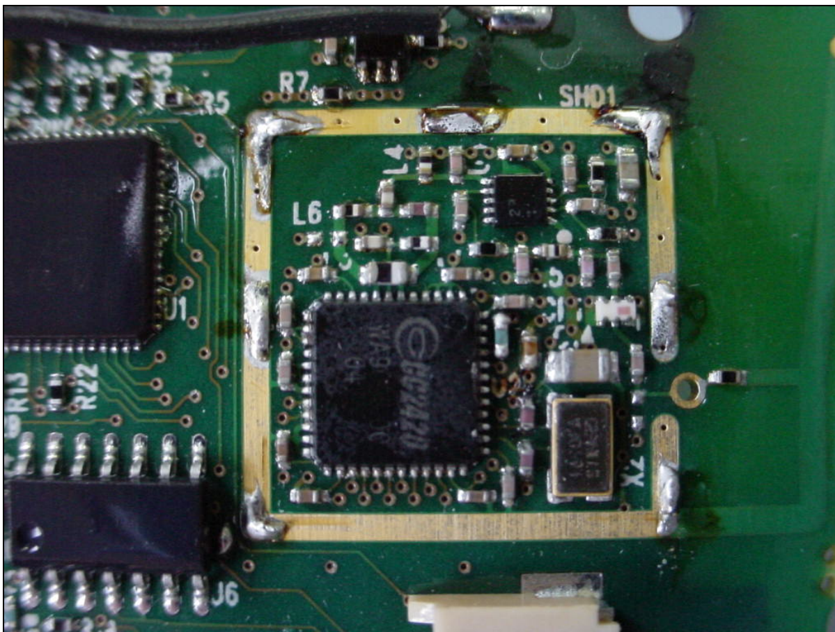
Photo Three – Internal Shield Removed. RF Section Close-Up
