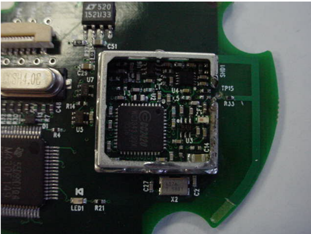
Photo Five – Internal Close-Up of RF Section
