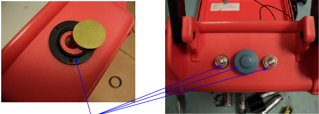
FIGURE 1. APPLY RTV (ITEM 28) TO PLASTIC CASE INSIDE O RING GASKET, UNDER LED'S AND RUBBER SWITCH BOOT PRIOR TO FINAL ASSEMBLY
