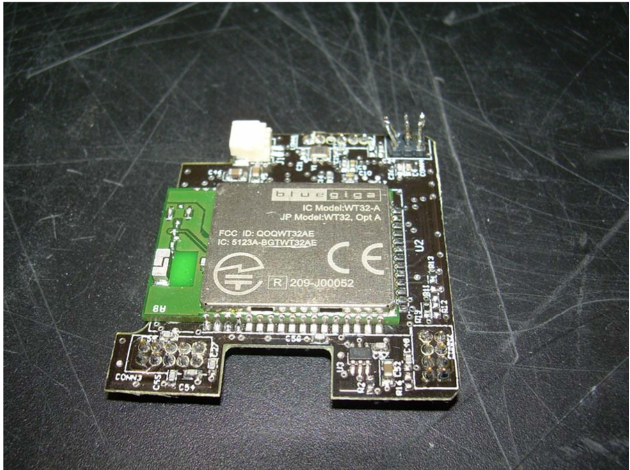
View of the RF PCB with Bluegiga Module
