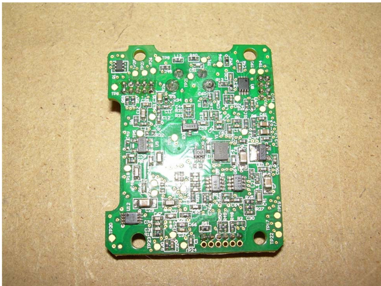
Bottom View of the Audio PCB
