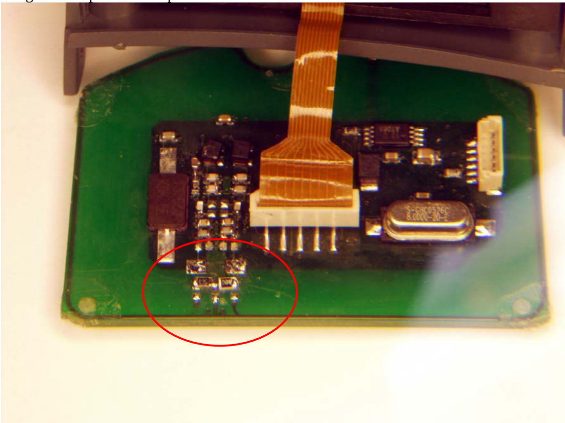
Integrated loop-antenna replaced with 50 \Omega load:
