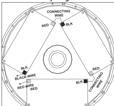
Battery Diagram
