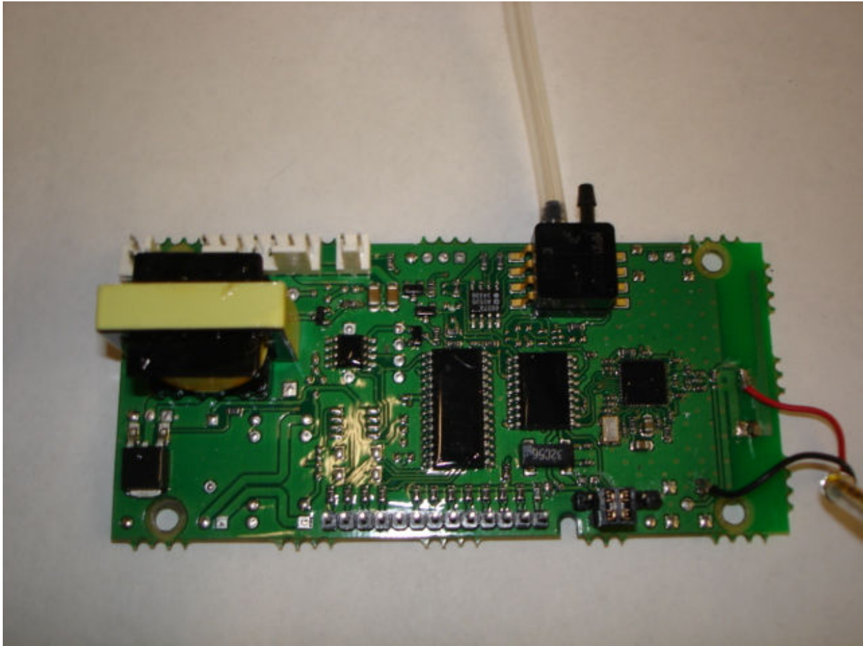
Detector unit, Transceiver Component side
