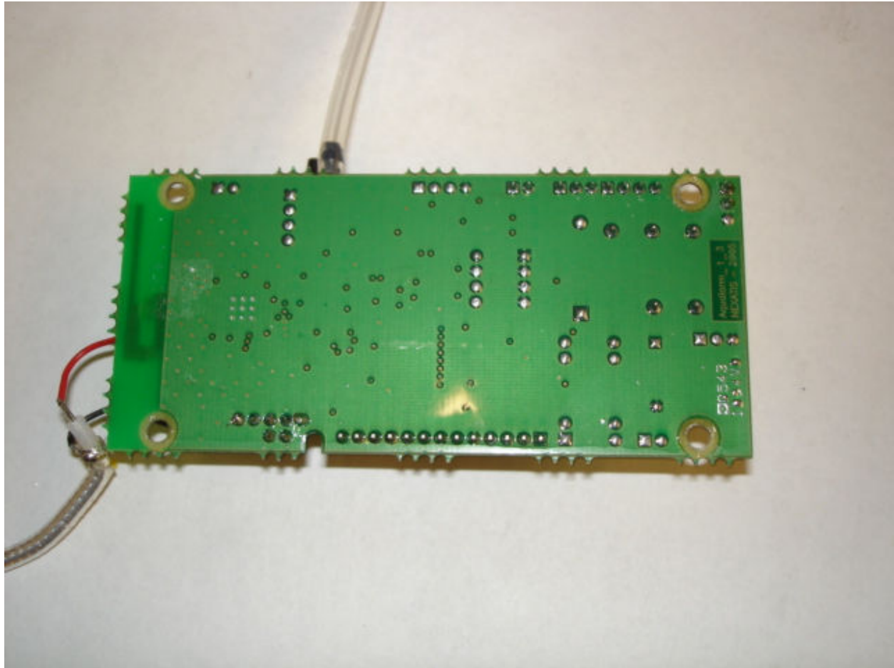
Detector unit, Transceiver PCB
