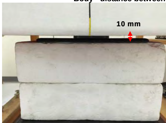
Fig.7 EUT Back side to flat phantom
