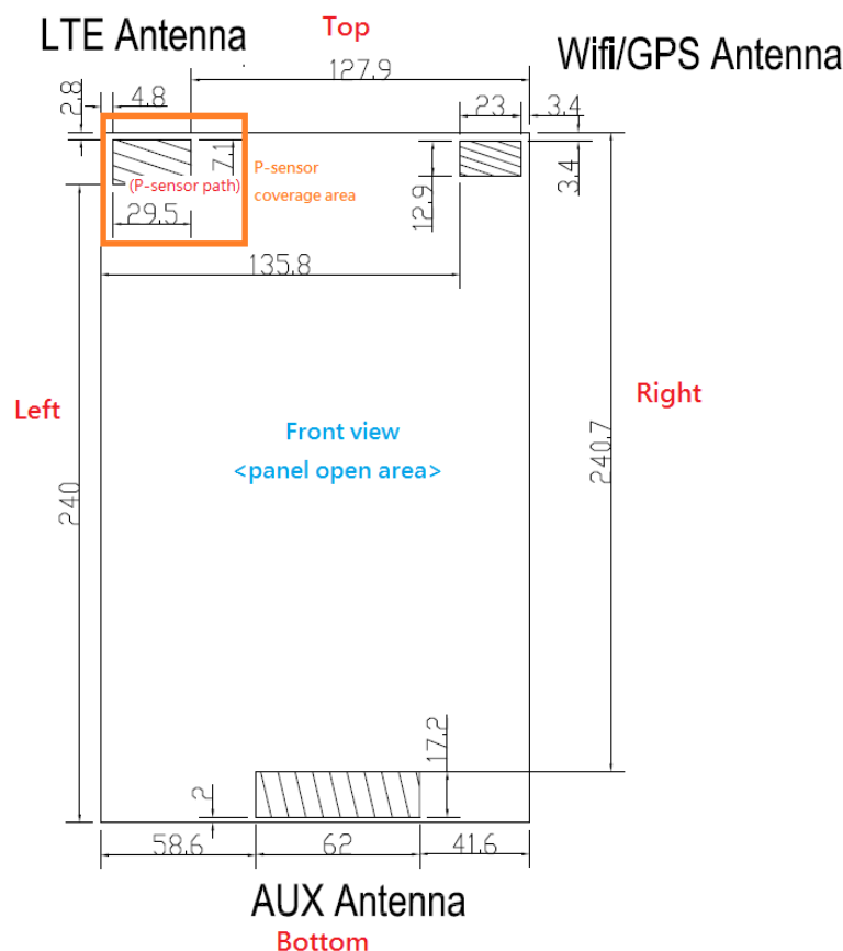
Fig.11 Antenna position of EUT (Front view)
