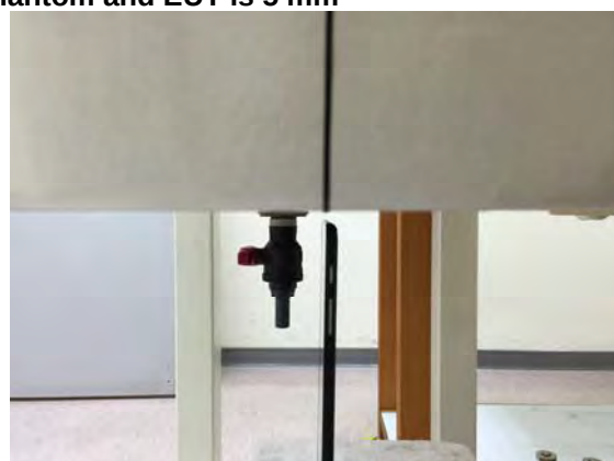
Fig.8 EUT Top side to flat phantom
