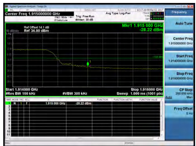
Band Edge_Band25_10MHz_QPSK_50_0_HighCH26640-1910
