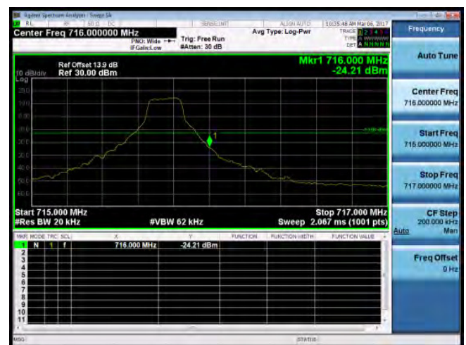
Band Edge_Band12_1.4MHz_QPSK_1_5_HighCH23173-715.3
