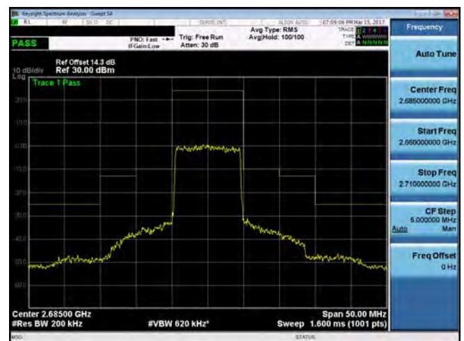
Emission Mask_Band 41_10M_QPSK_HIGH_RB50,0
