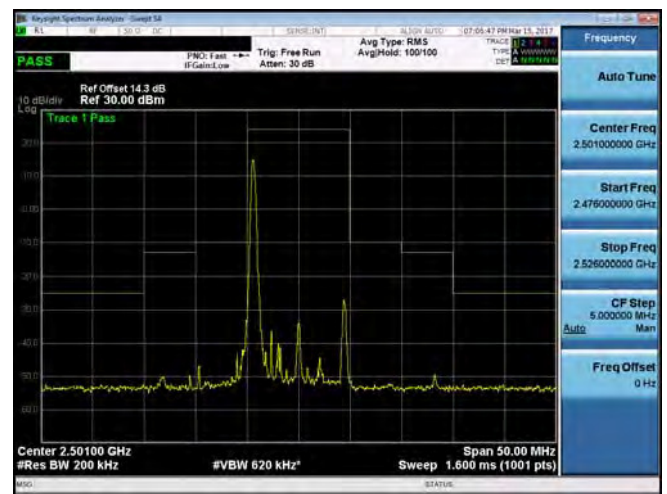
Emission Mask_Band 41_10M_QPSK_MID_RB1,0
