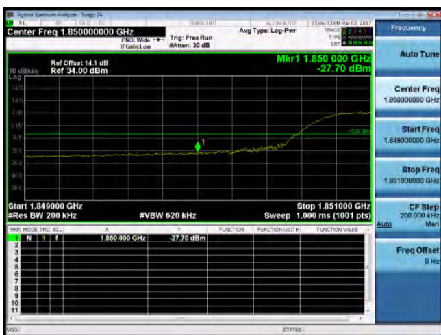
Band Edge_Band25_15MHz_QPSK_75_0_LowCH26115-1857.5
