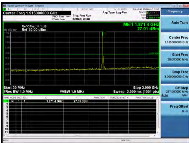
30MHz-3GHz_Band2_20MHz_QPSK_1_0_MidCH18900-1880
