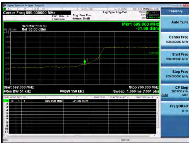
Band Edge_Band12_5MHz_QPSK_25_0_LowCH23035-701.5
