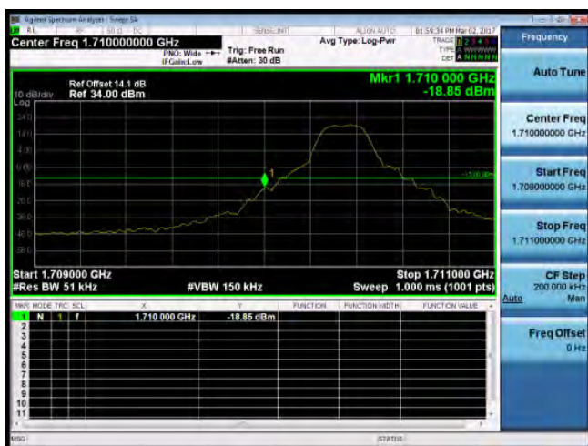
Band Edge_Band4_5MHz_QPSK_1_0_LowCH19975-1712.5
