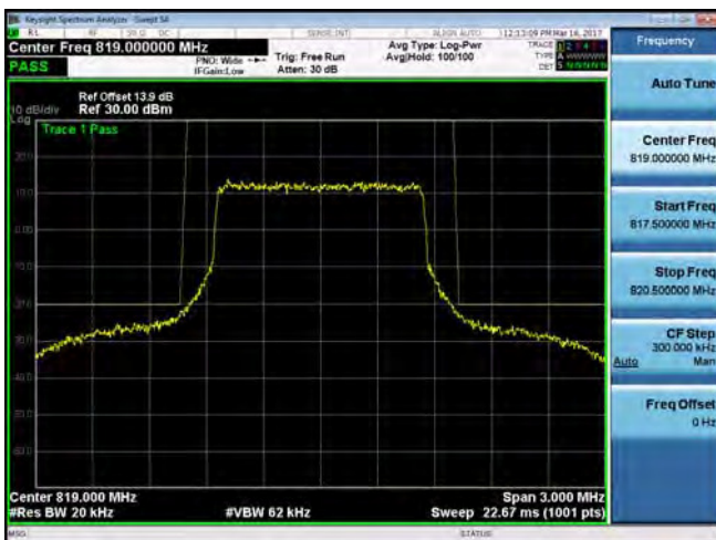
Emission Mask_Band26 for Part 90S_1.4M_QPSK_HIGH_RB6.0
