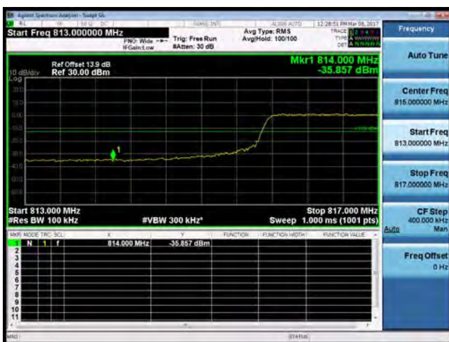
Band Edge_Band26_15MHz_QPSK_75_0_LowCH26775-822.5
