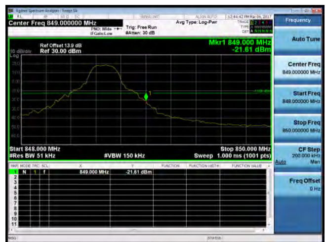
Band Edge_Band26_5MHz_QPSK_1_24_HighCH27015-846.5
