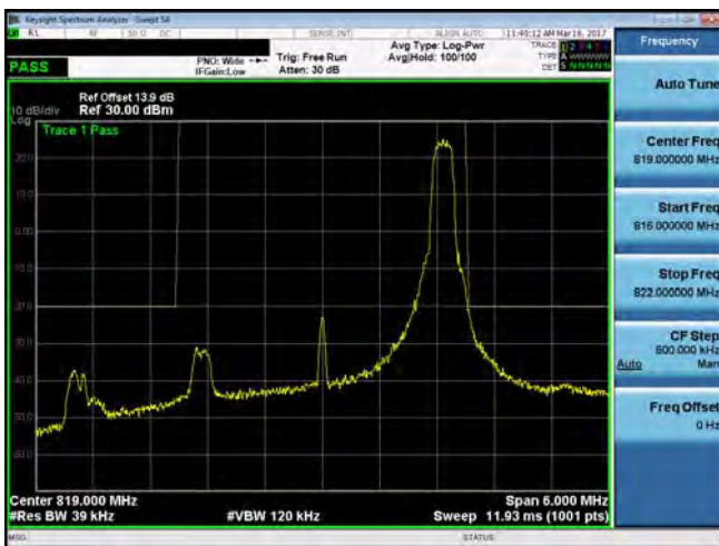
Emission Mask_Band26 for Part 90S_3M_QPSK_HIGH_RB1,14
