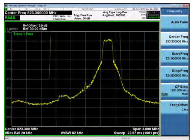
Emission Mask_Band26 for Part 90S_1.4M_QPSK_HIGH_RB1,5
