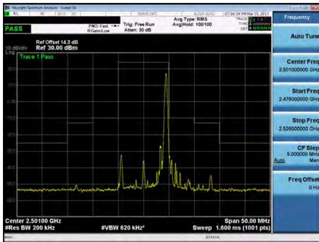
Emission Mask_Band 41_10M_QPSK_MID_RB1,49
