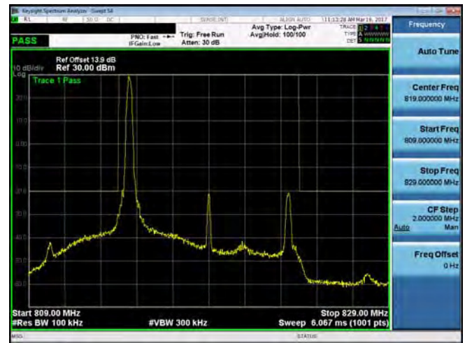
Emission Mask_Band26 for Part 90S_10M_QPSK_MID_RB1,49
