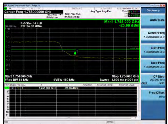
Band Edge_Band4_5MHz_QPSK_25_0_HighCH20375-1752.5
