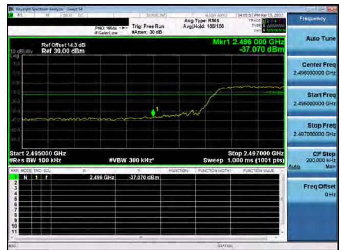
Band Edge_Band41_10MHz_QPSK_50_0_HighCH41540
