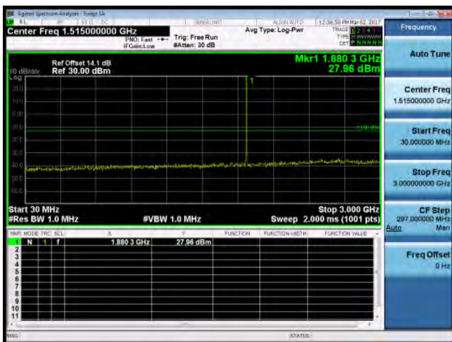
30MHz-3GHz_Band2_1.4MHz_QPSK_1_0_MidCH18900-1880
