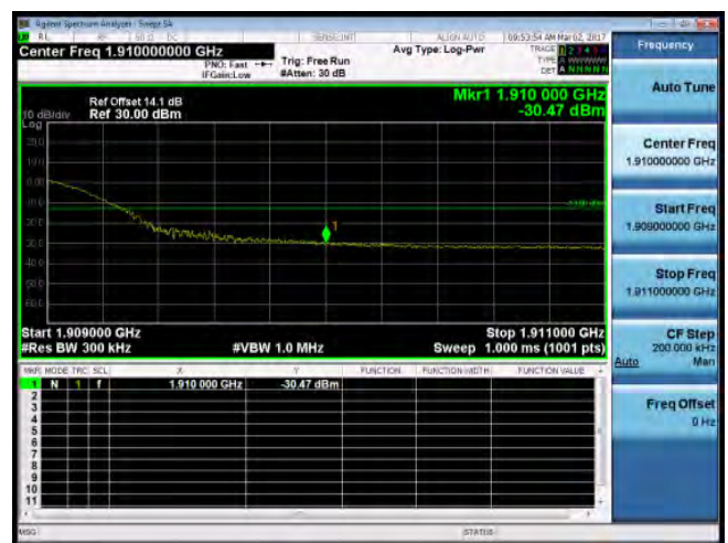
Band Edge_Band2_20MHz_QPSK_100_0_HighCH19100-1900
