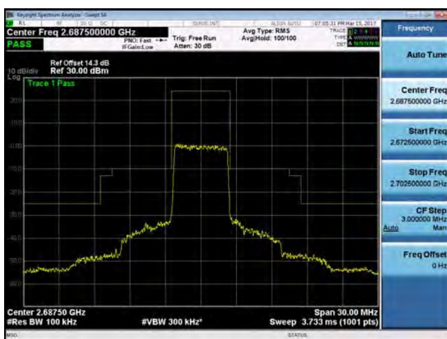
Emission Mask_Band 41_5M_QPSK_HIGH_RB25,0
