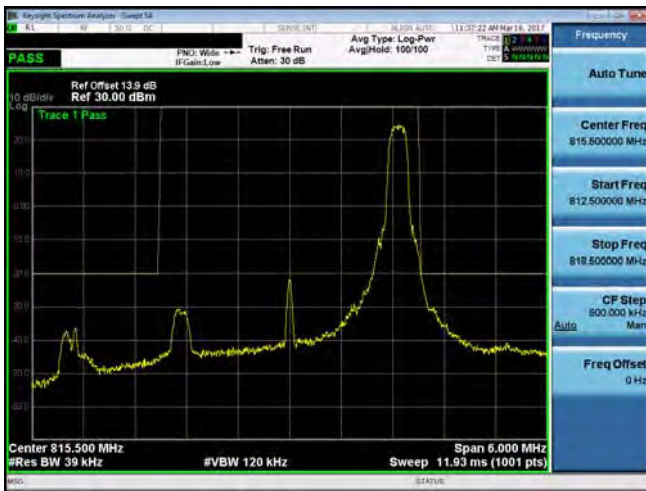
Emission Mask_Band26 for Part 90S_3M_QPSK_MID_RB1,14
