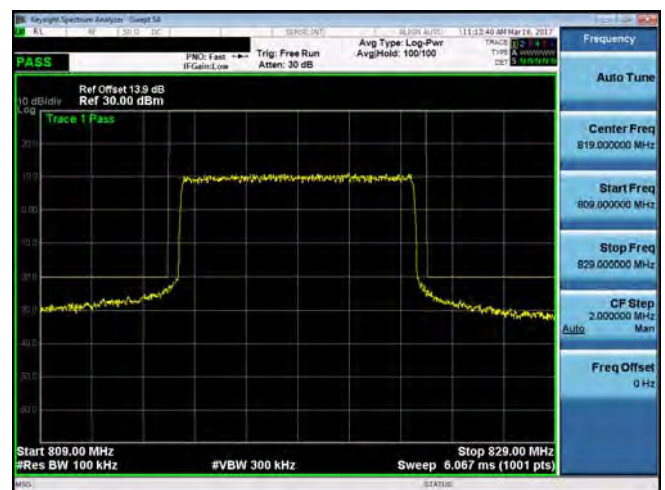
Emission Mask_Band26 for Part 90S_10M_QPSK_MID_RB50,0
