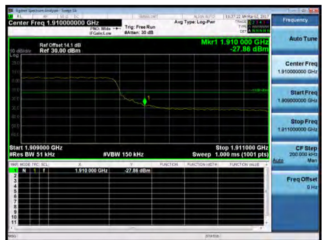
Band Edge_Band2_5MHz_QPSK_25_0_HighCH19175-1907.5
