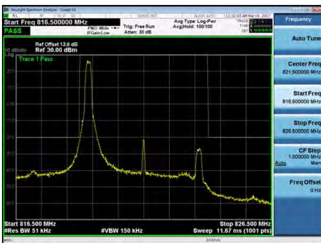
Emission Mask_Band26 for Part 90S_5M_QPSK_HIGH_RB1,0
