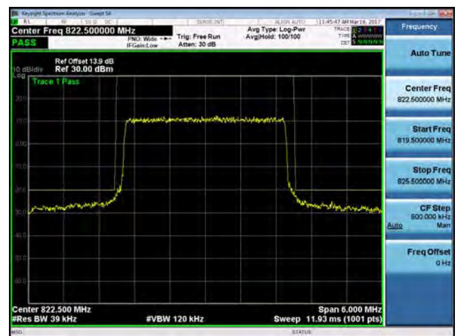
Emission Mask_Band26 for Part 90S_3M_QPSK_HIGH_RB15,0
