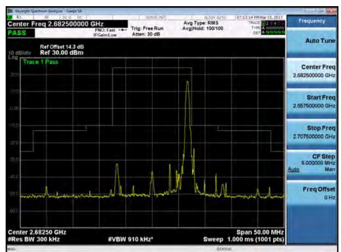
Emission Mask_Band 41_15M_QPSK_HIGH_RB1,74
