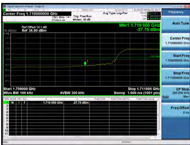
Band Edge_Band4_10MHz_QPSK_50_0_LowCH20000-1715
