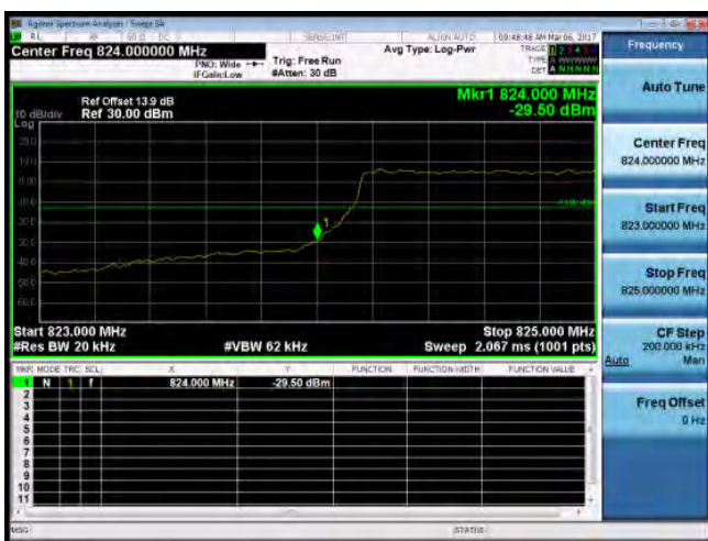
Band Edge_Band5_1.4MHz_QPSK_6_0_LowCH20407-824.7
