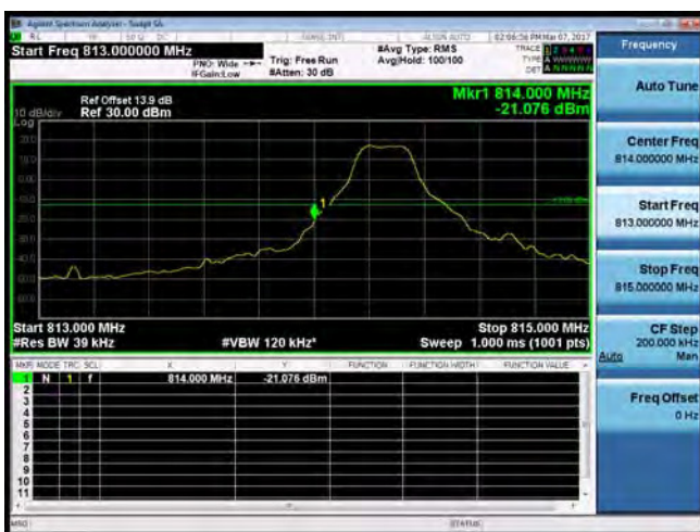
Band Edge_Band26_1.4MHz_QPSK_1_0_LowCH26697-814.7
