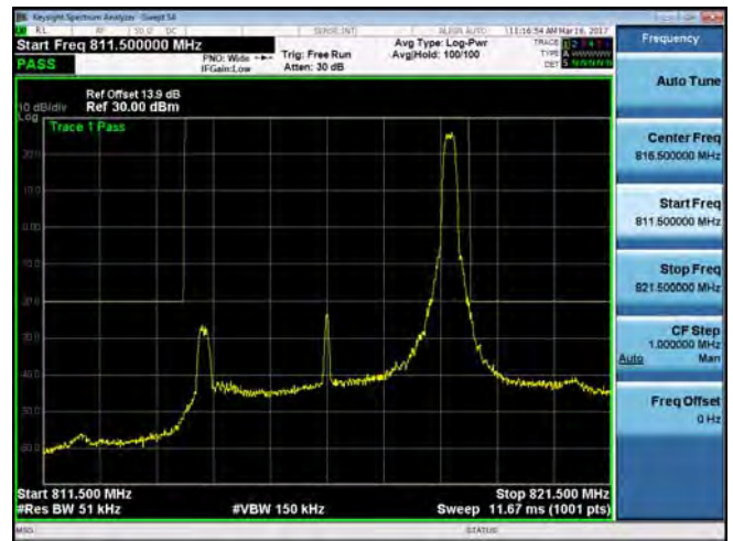
Emission Mask_Band26 for Part 90S_5M_QPSK_MID_RB1,24
