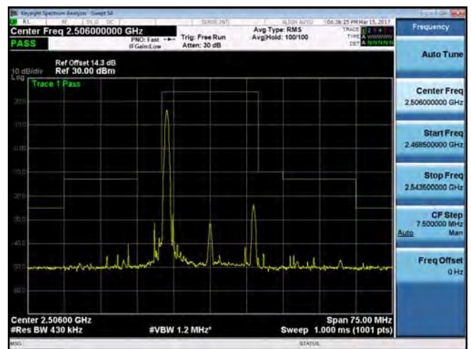
Emission Mask_Band 41_20M_QPSK_MID_RB1,0
