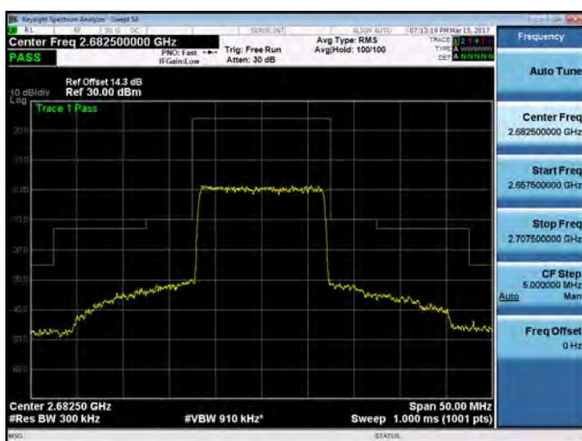
Emission Mask_Band 41_15M_QPSK_HIGH_RB75,0
