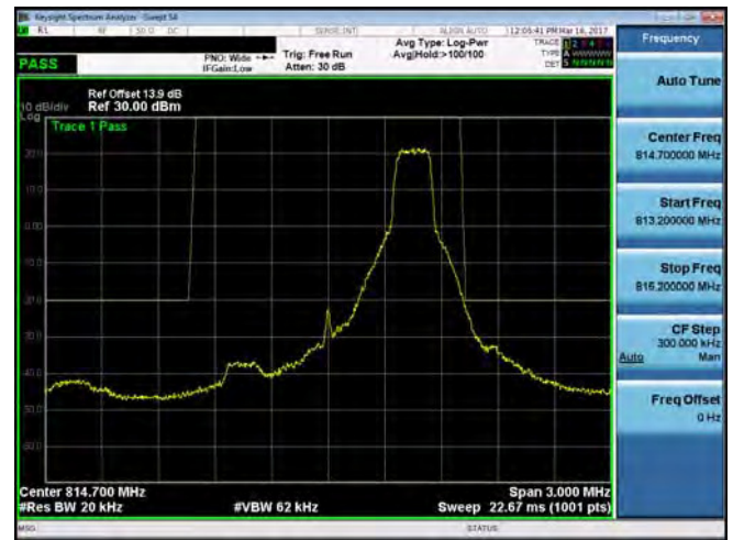
Emission Mask_Band26 for Part 90S_1.4M_QPSK_MID_RB1,5
