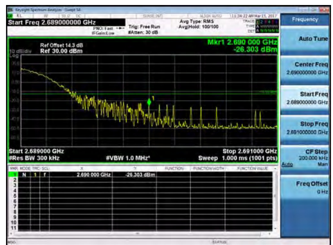
Band Edge_Band41_20MHz_QPSK_1_99_HighCH41490
