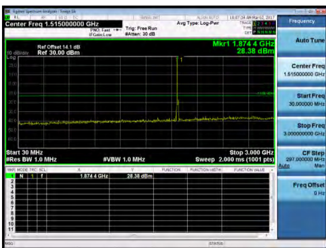
30MHz-3GHz_Band2_15MHz_QPSK_1_0_MidCH18900-1880
