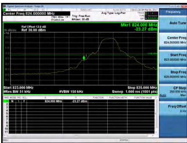
Band Edge_Band5_5MHz_QPSK_1_0_LowCH20425-826.5
