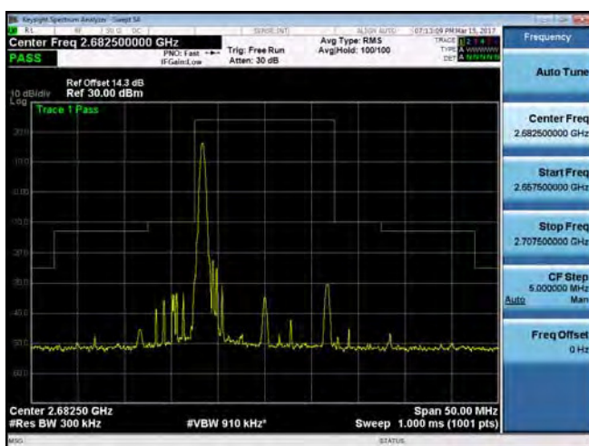
Emission Mask_Band 41_15M_QPSK_HIGH_RB1,0
