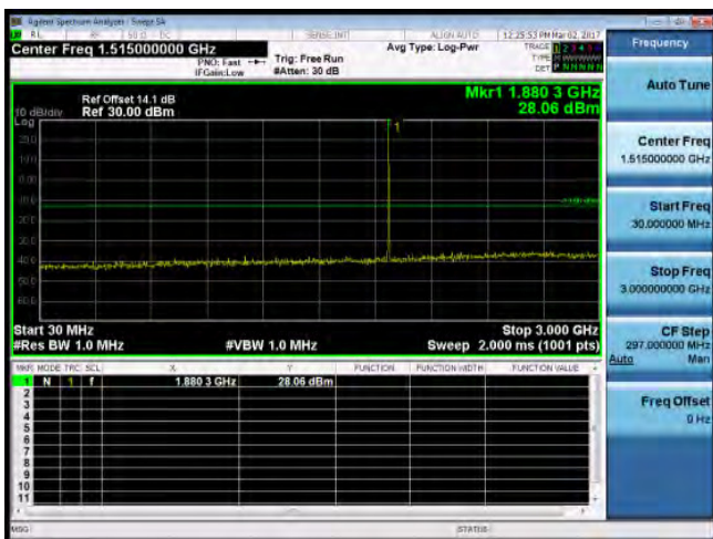
30MHz~3GHz_Band2_3MHz_QPSK_1_0_MidCH18900-1880
