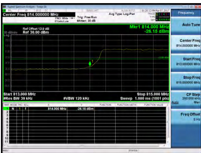
Band Edge_Band26_3MHz_QPSK_15_0_LowCH26705-815.5
