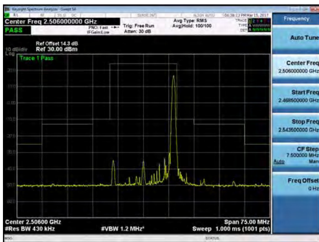
Emission Mask_Band 41_20M_QPSK_MID_RB1,99
