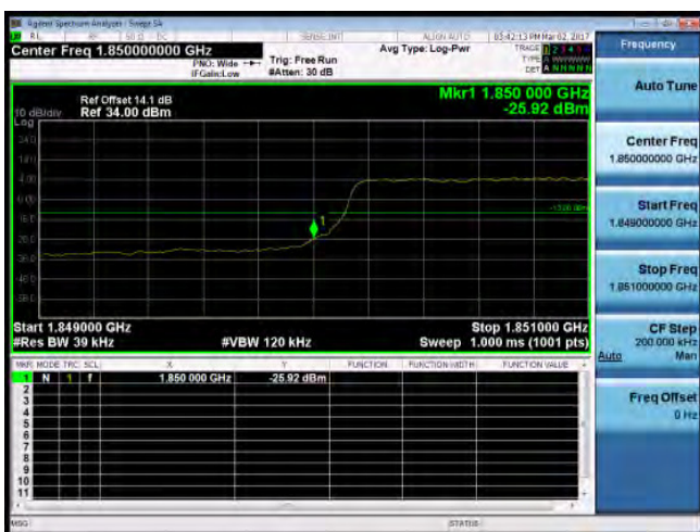
Band Edge_Band25_3MHz_QPSK_15_0_LowCH26055-1851.5
