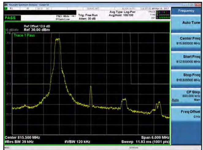
Emission Mask_Band26 for Part 90S_3M_QPSK_MID_RB1,0
