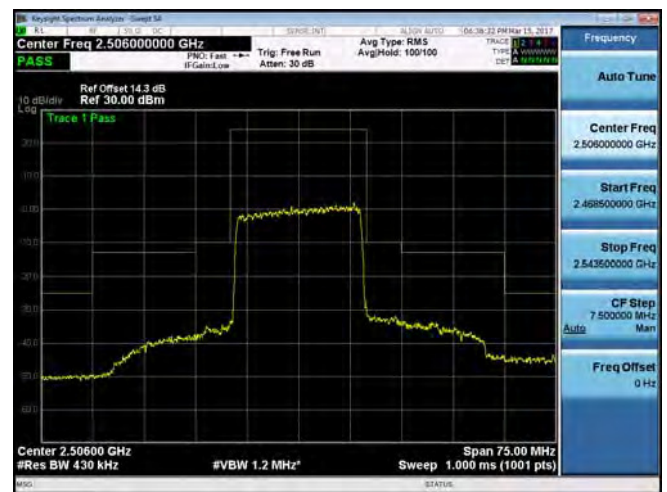
Emission Mask_Band 41_20M_QPSK_MID_RB100,0
