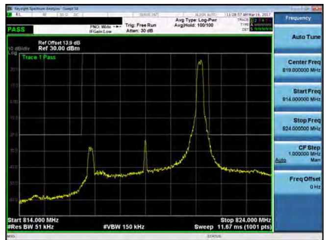
Emission Mask_Band26 for Part 90S_5M_QPSK_HIGH_RB1,24
