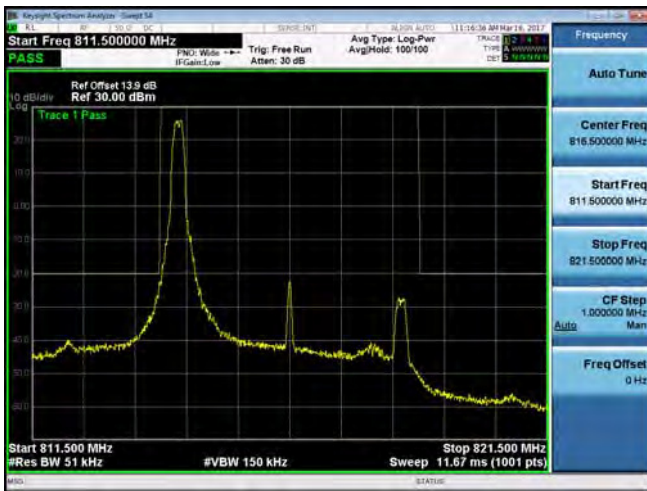
Emission Mask_Band26 for Part 90S_5M_QPSK_MID_RB1,0
