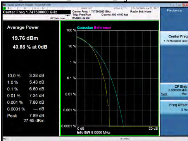
LTE_Band4 15MHz_16-QAM 75 0_HighCH20325-1747.5
