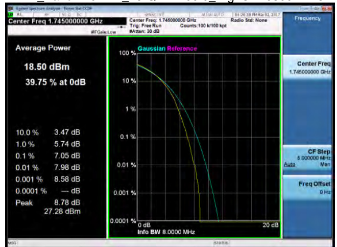
LTE_Band4 20MHz_16-QAM 100 0_HighCH20300-1745
