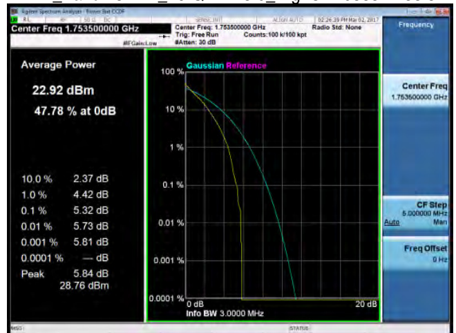
LTE_Band4 3MHz_16-QAM 15 0_HighCH20385-1753.5
