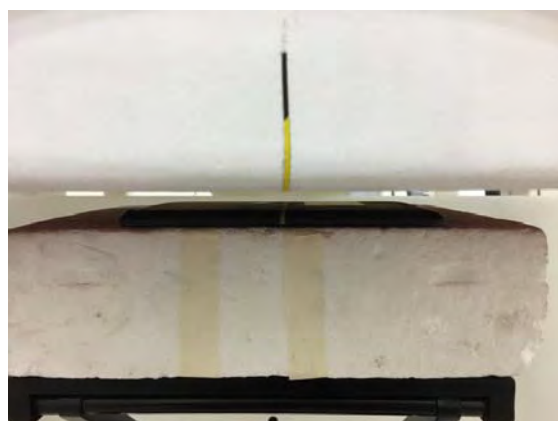
Fig.4 EUT Back side (15mm) to flat phantom
