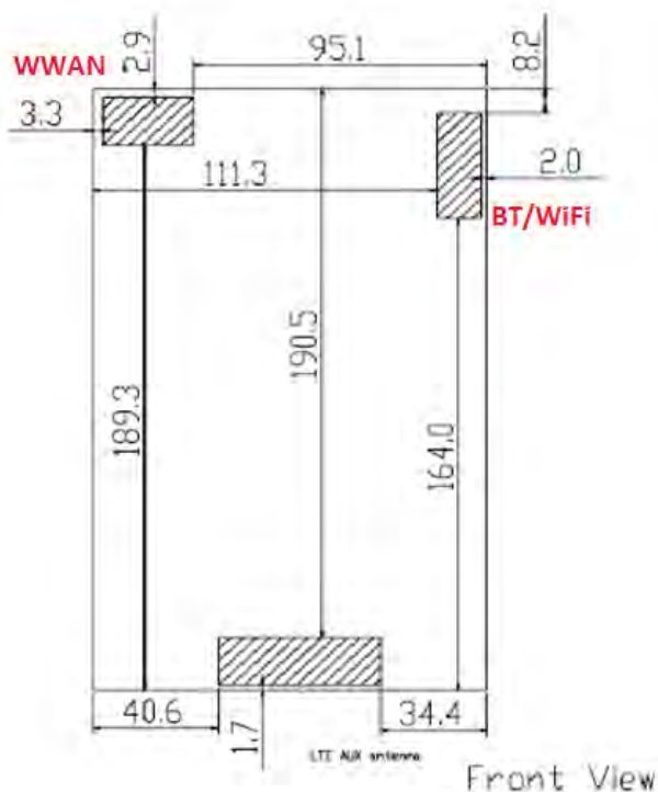
Fig.14 Antenna position of EUT (Front view)
