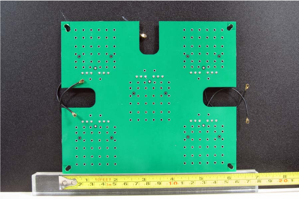
DECT Antenna Rear
