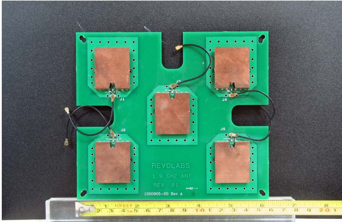
DECT Antenna – Front
