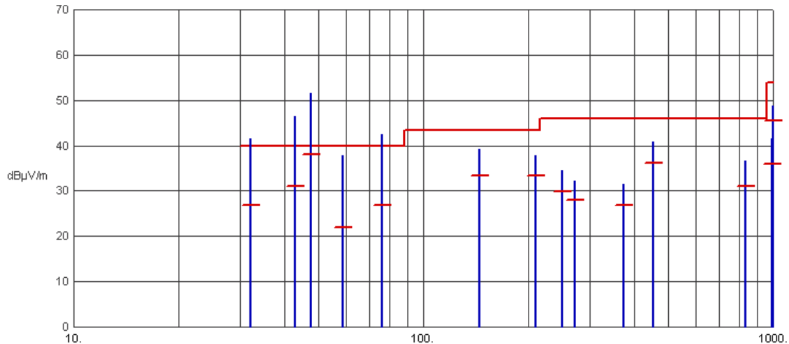
Test No.: 165-14, Radiated Emissions - Vertical Polarity
