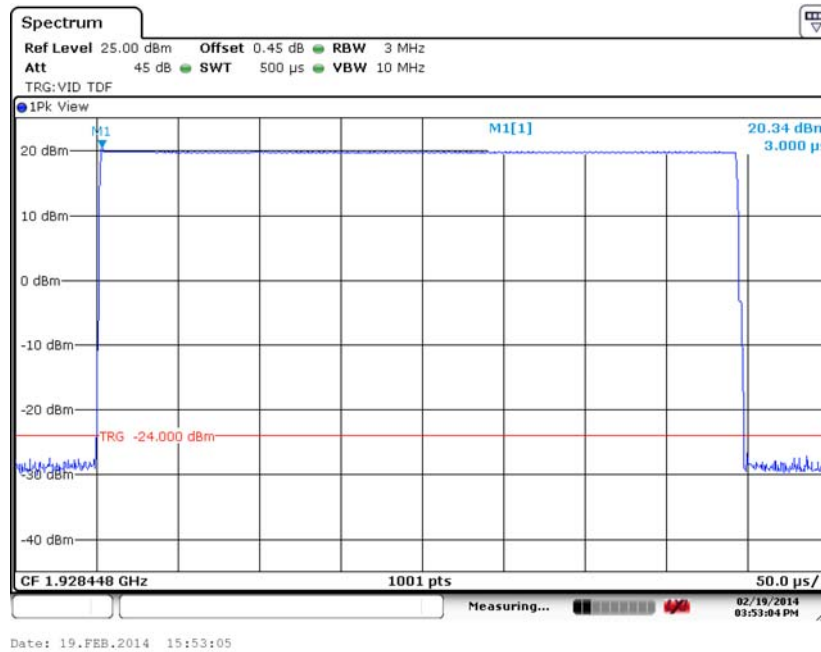
Channel 0 – BB3
