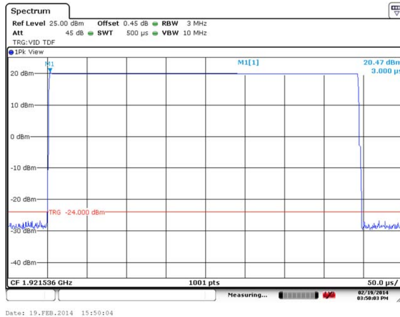
Channel 4 – BB3
