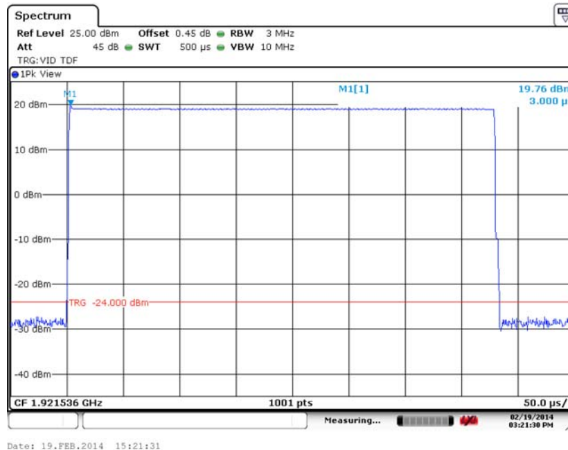
Channel 4 – BB2
