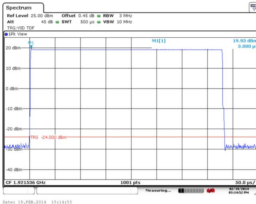
Channel 4 – BB1
