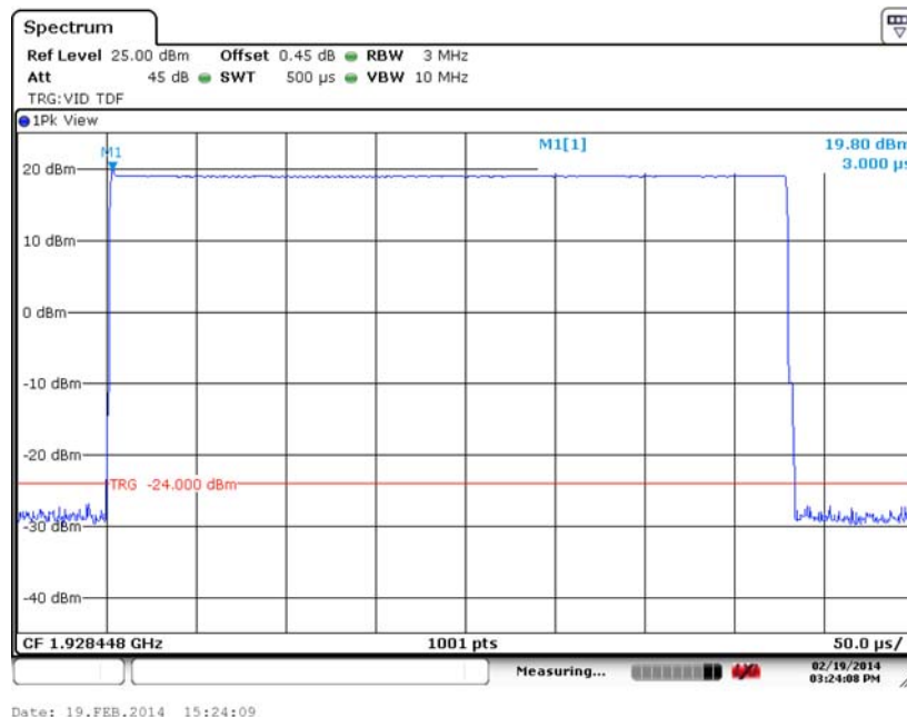
Channel 0 – BB2
