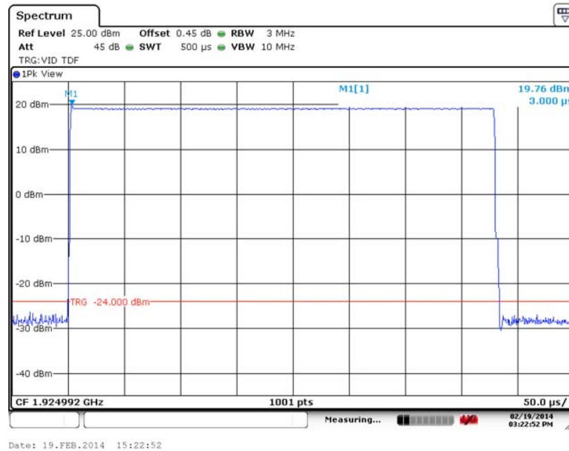
Channel 2 – BB2
