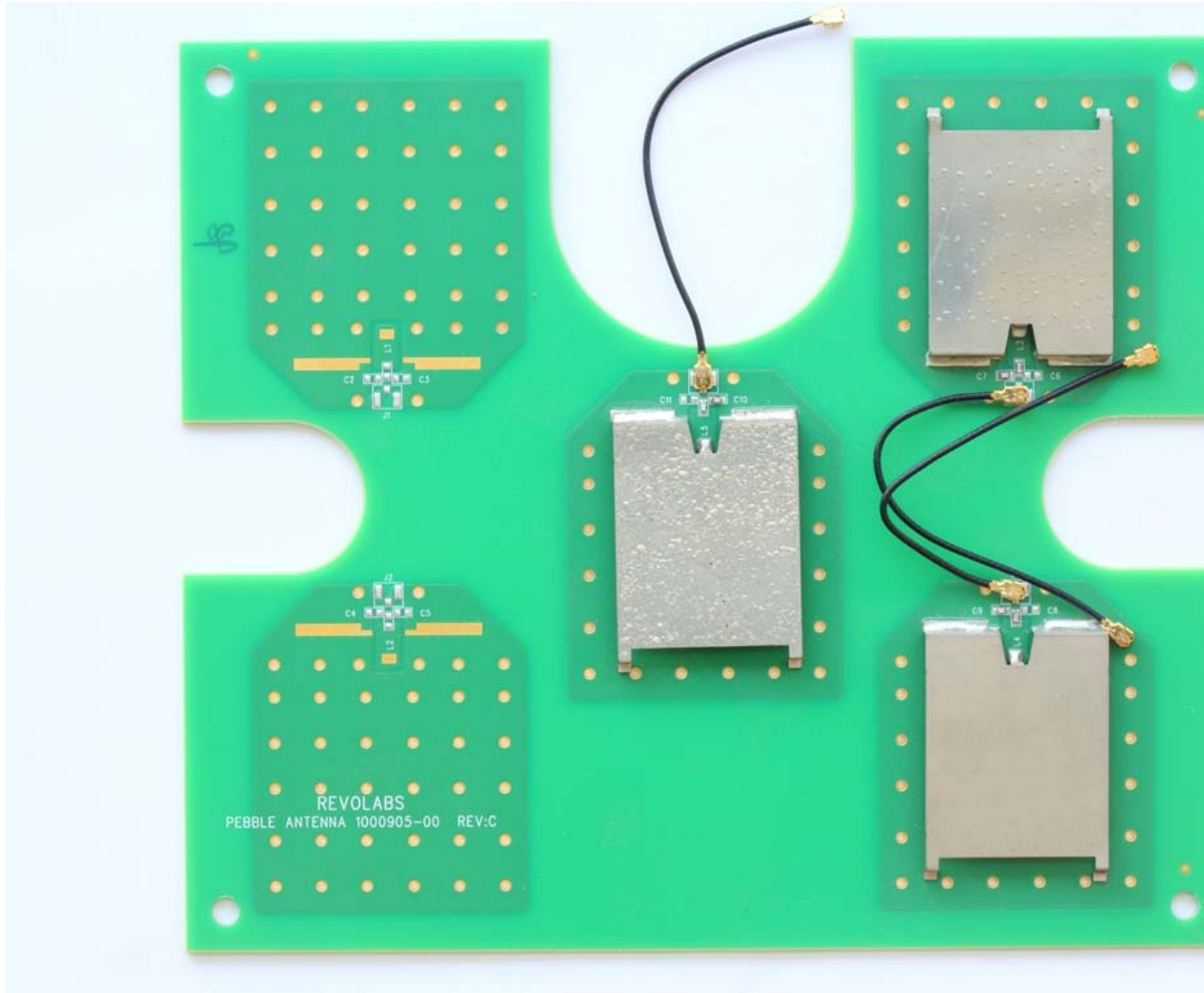
Antenna Board component side
