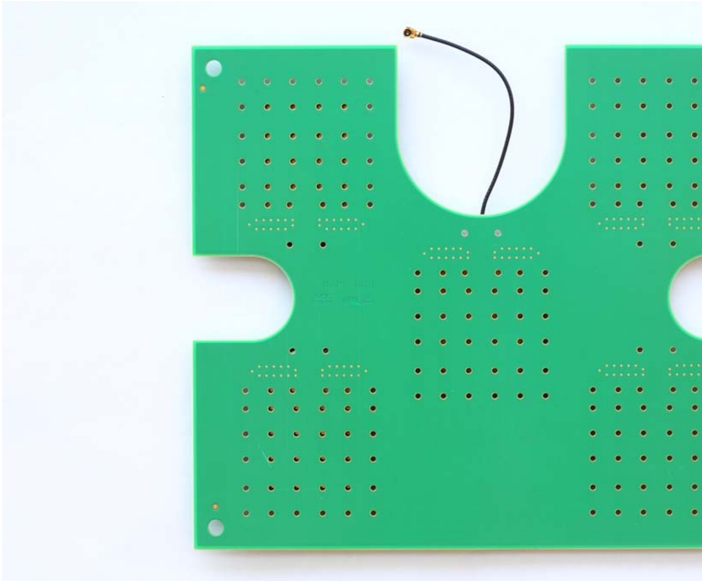
Antenna board solder side
