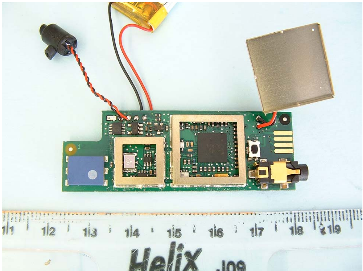
Solo Executive Microphone Main PCB RF Side Can Lids Removed
