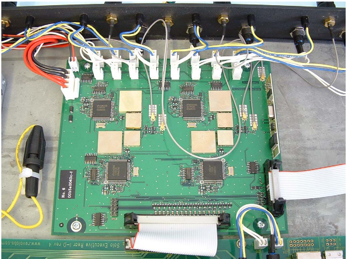
Solo Executive Base Station - Close-up of Board
