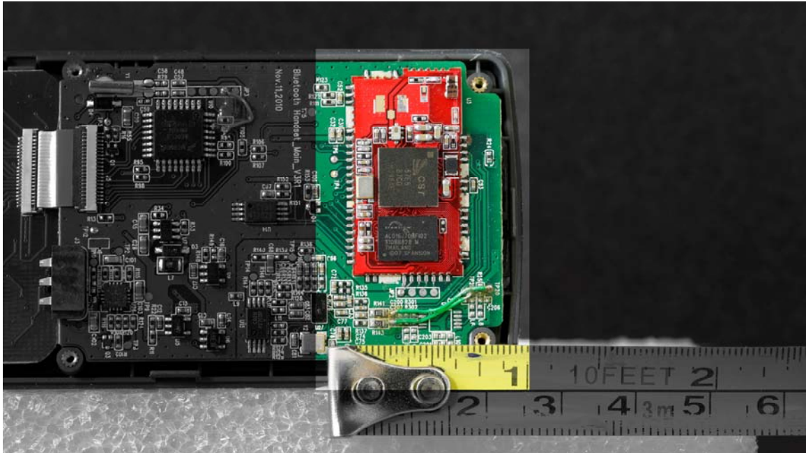
Transmitter Module close up
