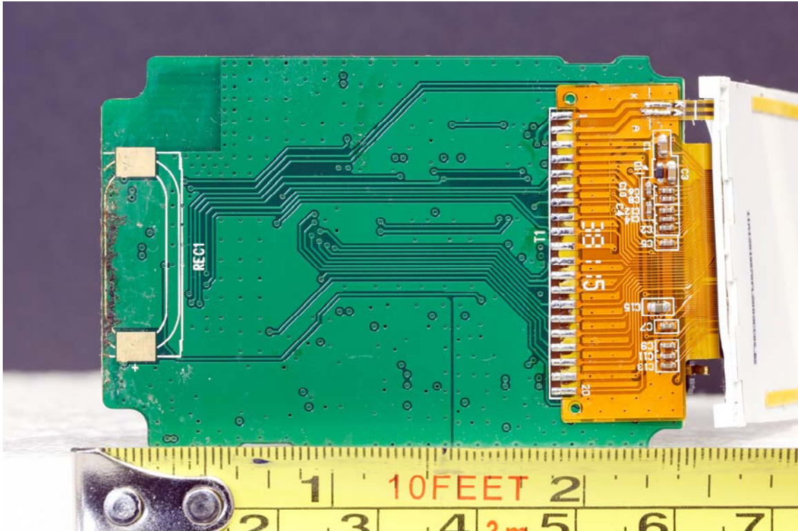
Main Board – Back Side – No cable
