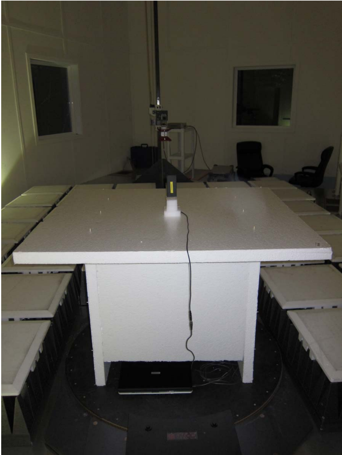
Microwave Emissions Rear View
