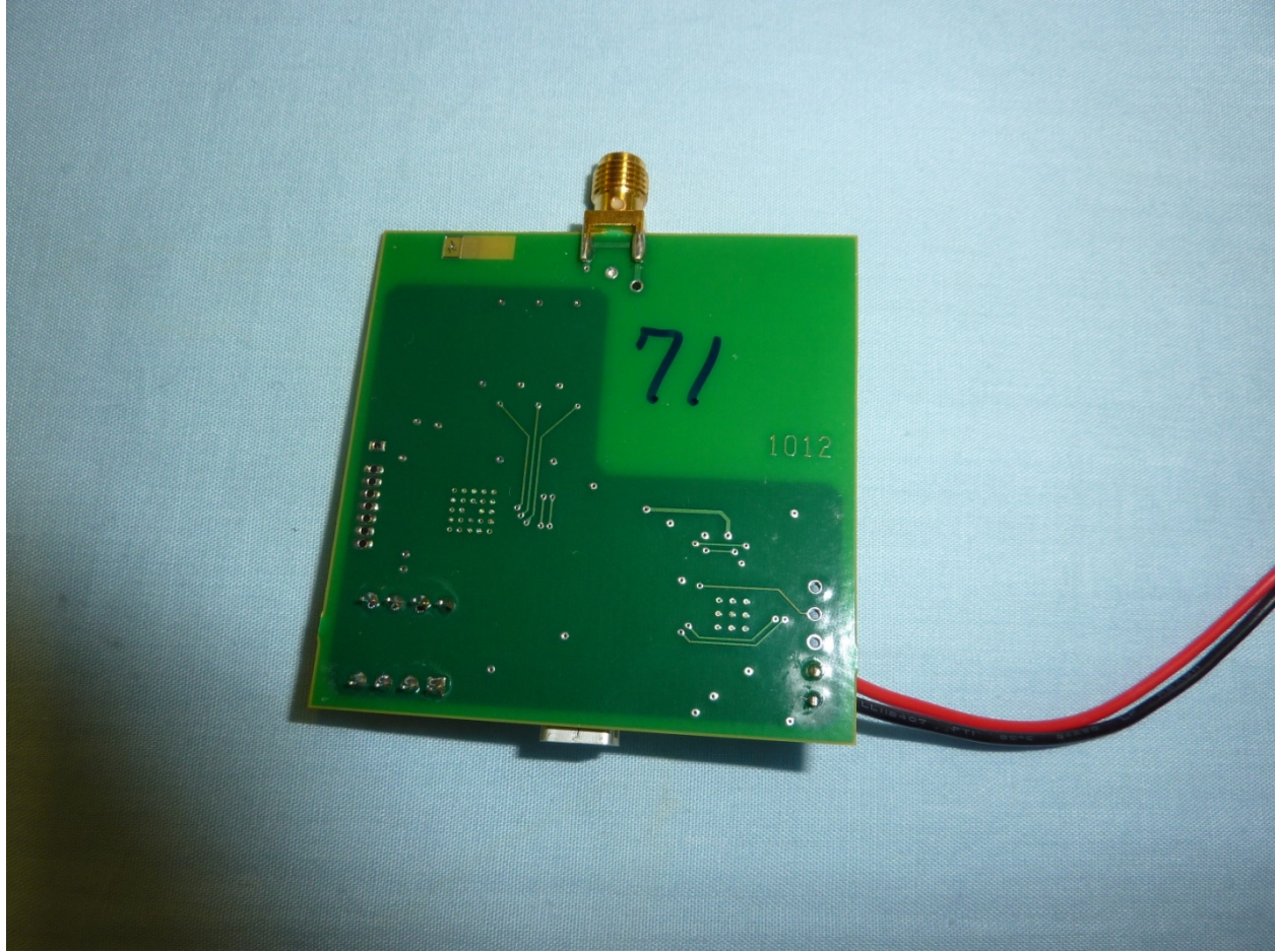
EUT with Test Jig Back side View
