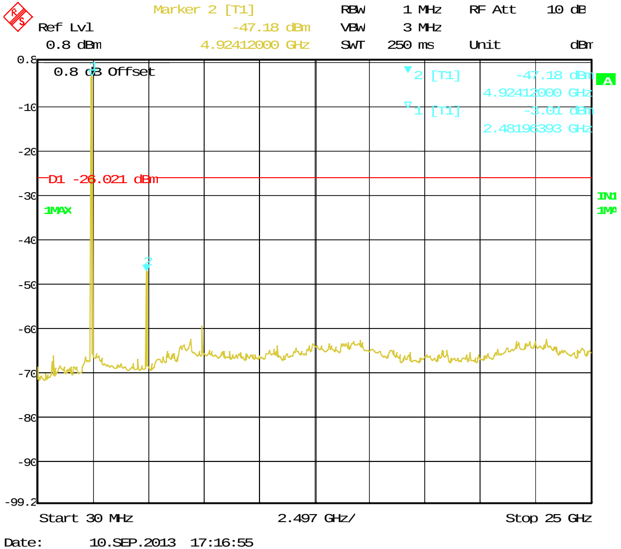
Figure 18: Out of band emissions at Operating Channel 2480 MHz
