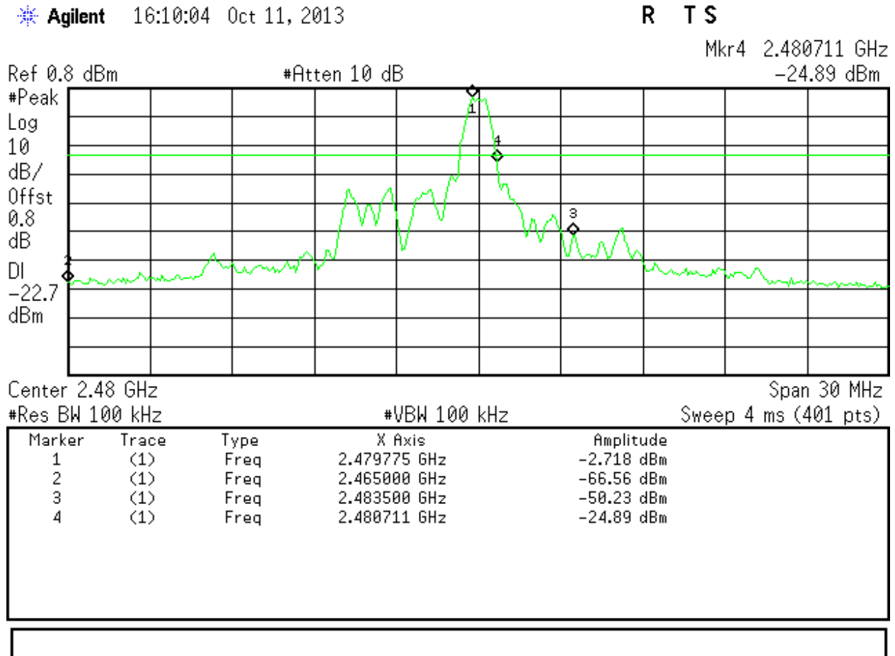
Figure 15: Band Edge Requirement at Operating Channel 2480 MHz
