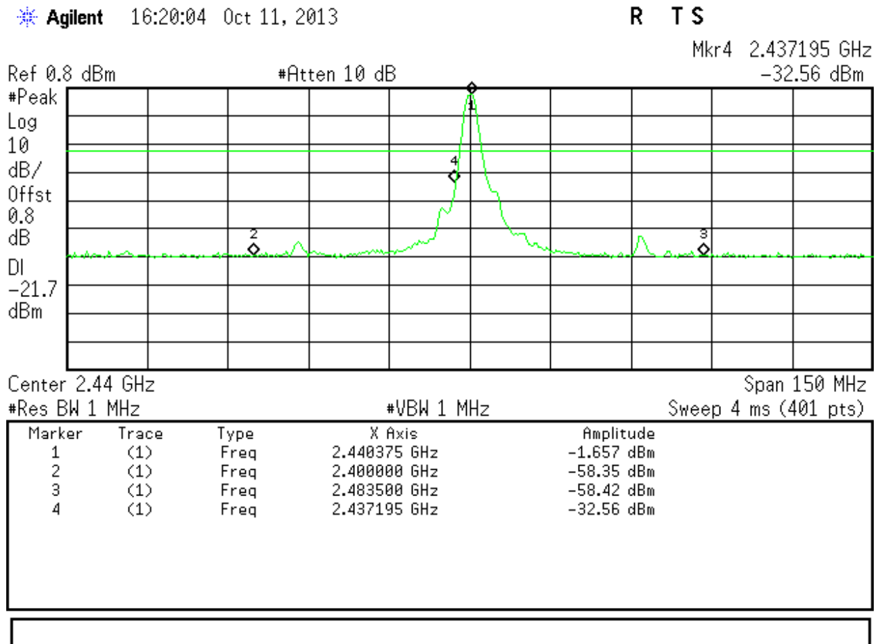
Figure 14: Band Edge Requirement at Operating Channel 2440 MHz
