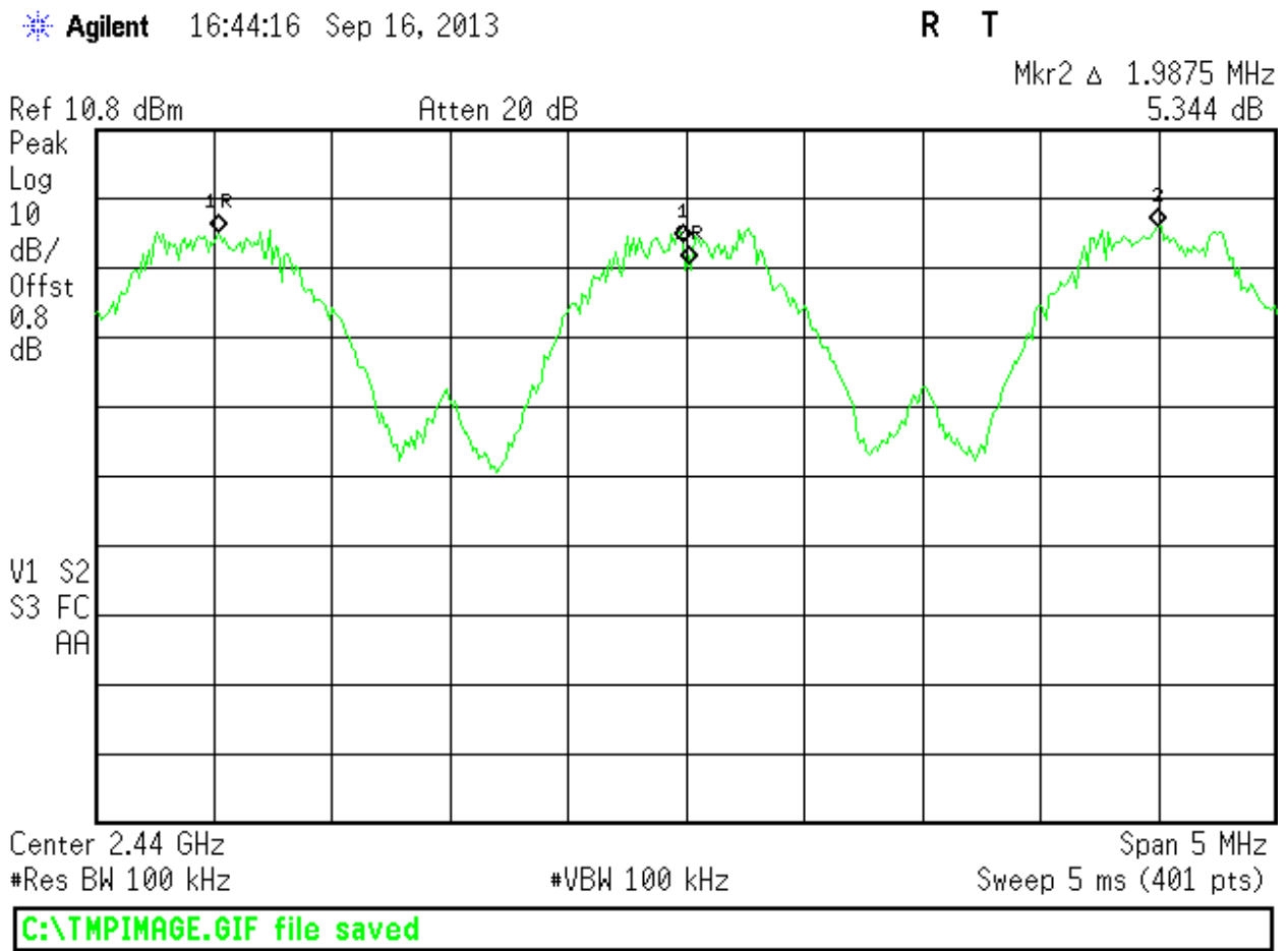
Figure 9: Channel Sepeation, plot 2
