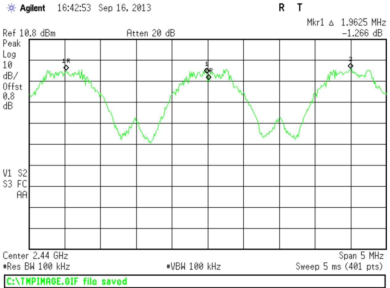
Figure 8: Channel Sepeation, plot 1
