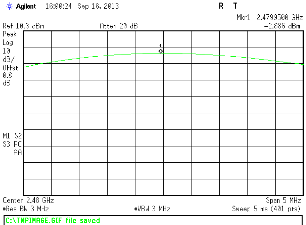
Figure 3: Maximum Transmitted Power, 2480 MHz, 1 Mbps
