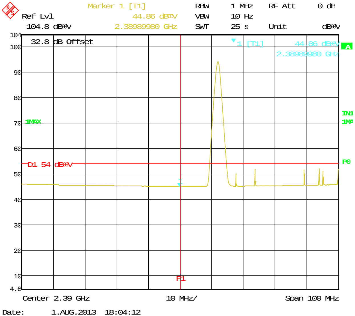
Figure 20: Radiated Emission at the Edge for Channel 2402 MHz at 1Mbps – Horizontal (Avg)
