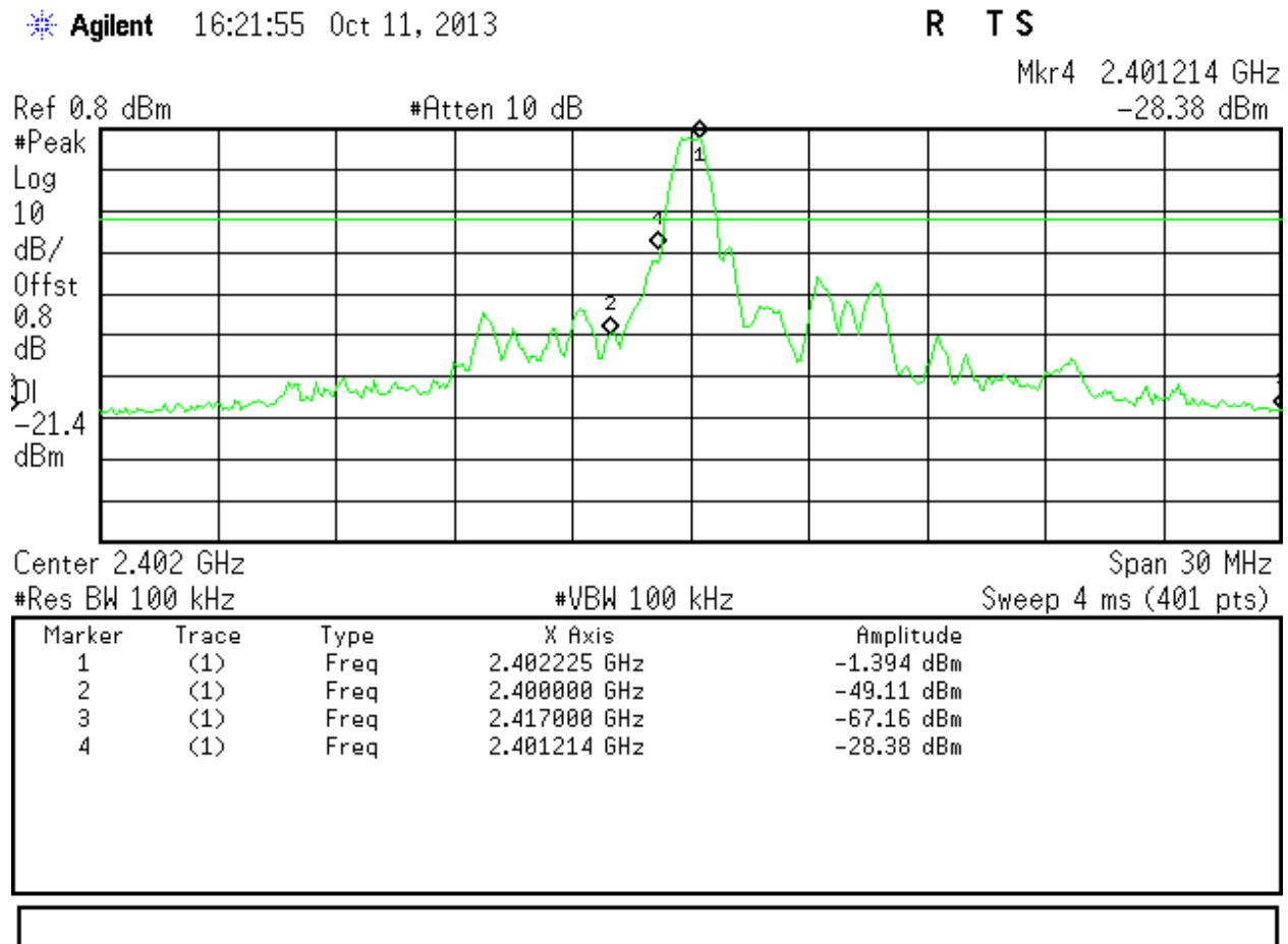
Figure 13: Band Edge Requirement at Operating Channel 2402 MHz
