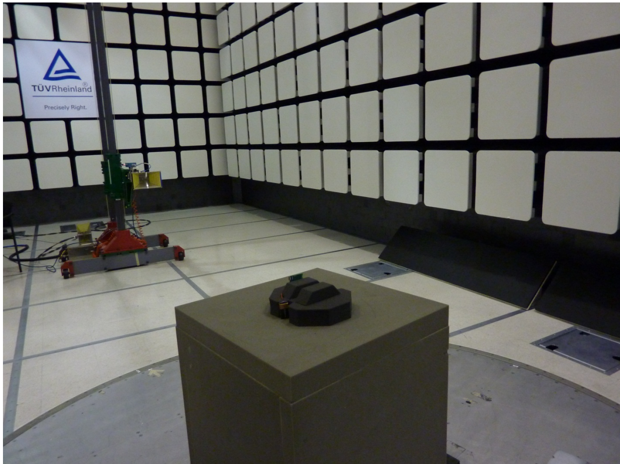
Radiated Emissions 1 to 18GHz
