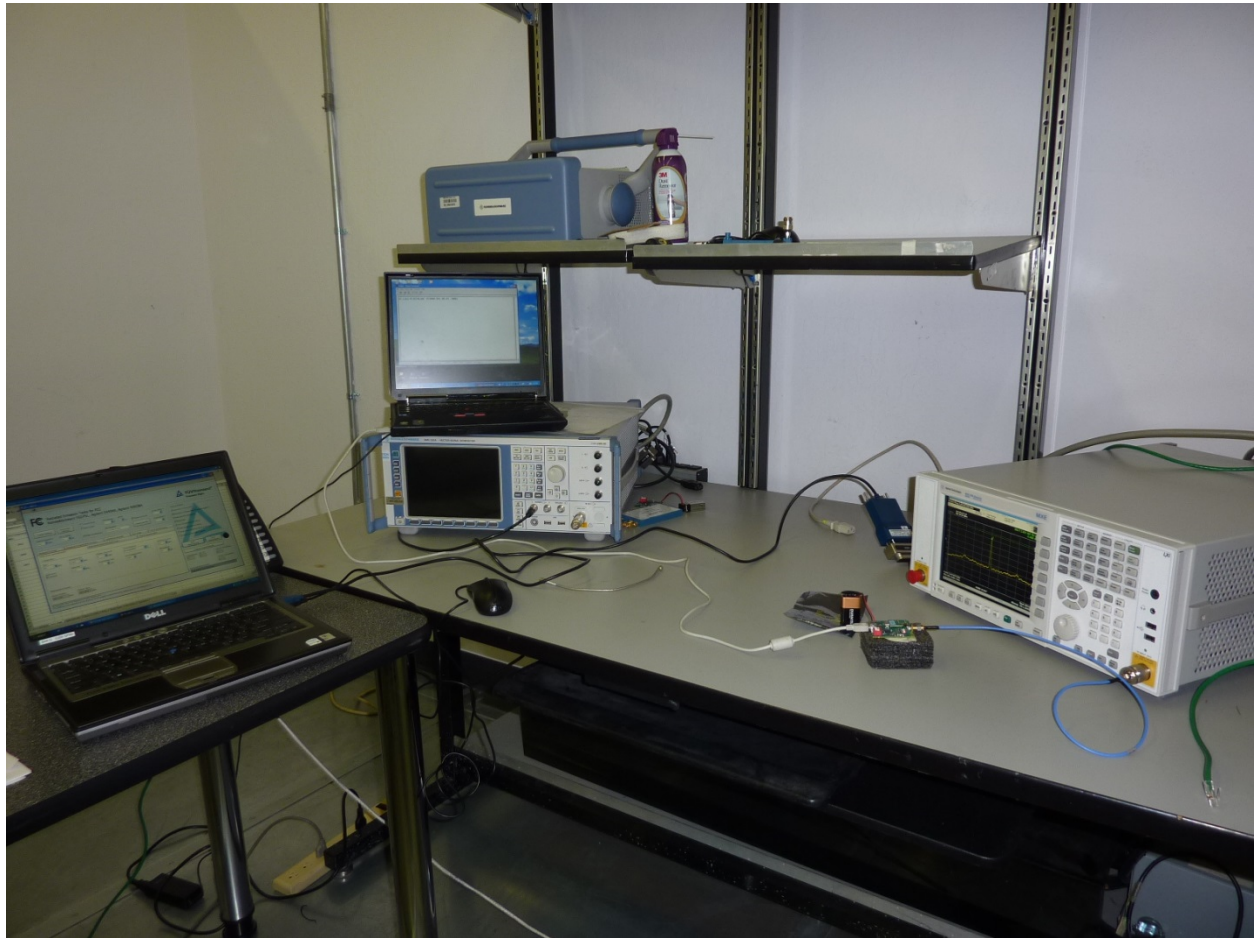
Test setup Conducted TX measurements
