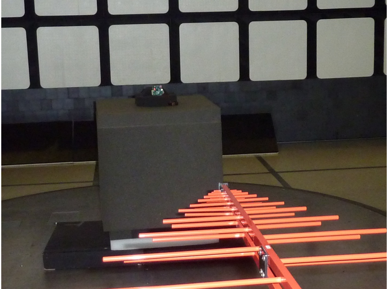
Radiated Emissions 30 to 1000MHz
