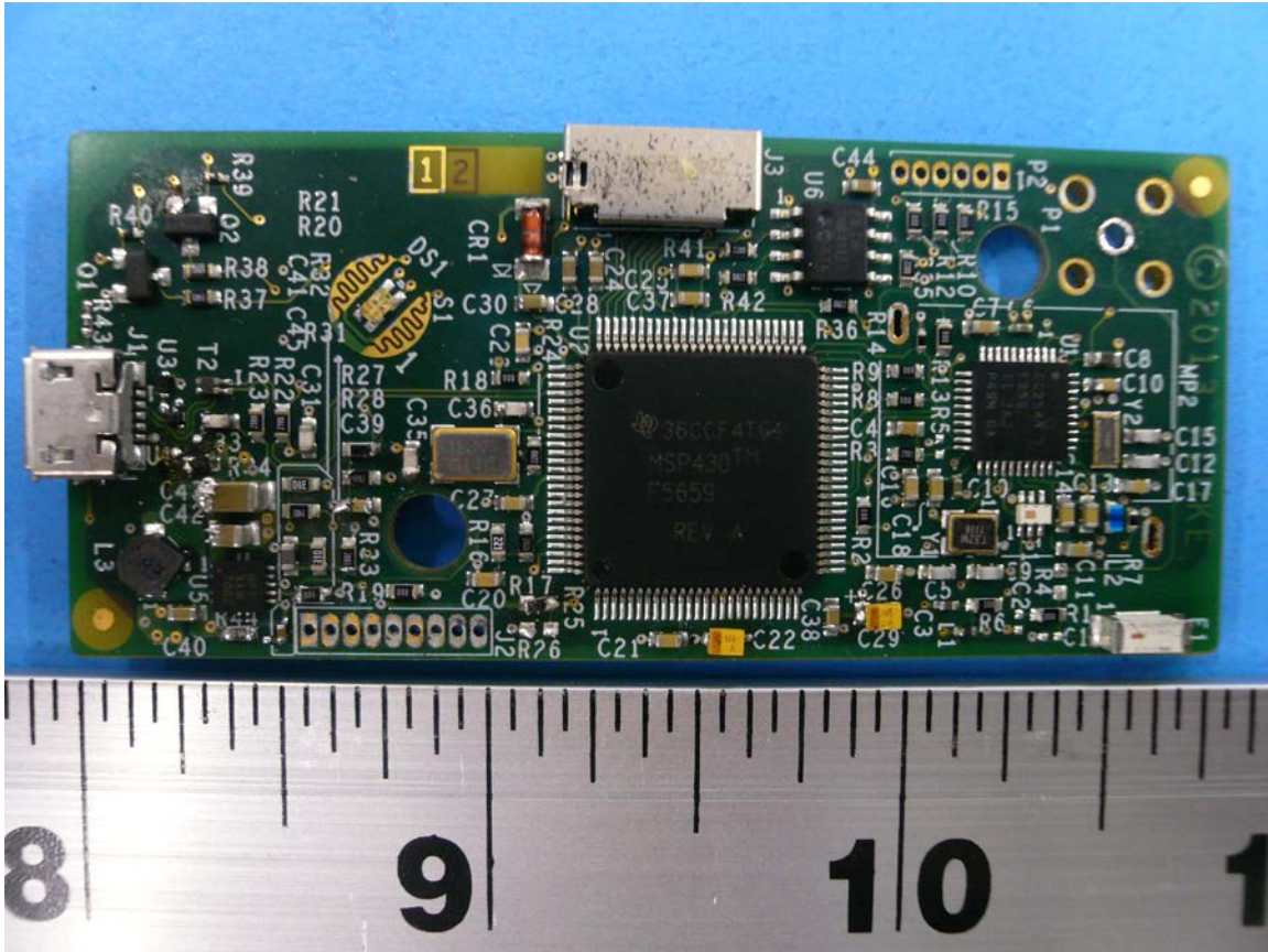
Figure 1: pc3000 FC Main PCB – Top Side
