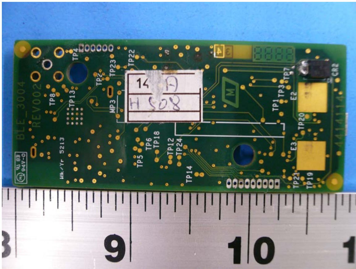
Figure 2: ir3000 FC Main PCB – Bottom Side
