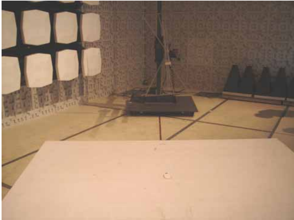
Radiation Emission Test View for 1GHz -5GHz
