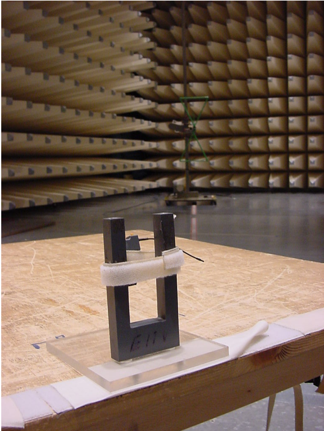
Photo 3 (Radiated Emissions): Tx with Lambda/8 antenna
