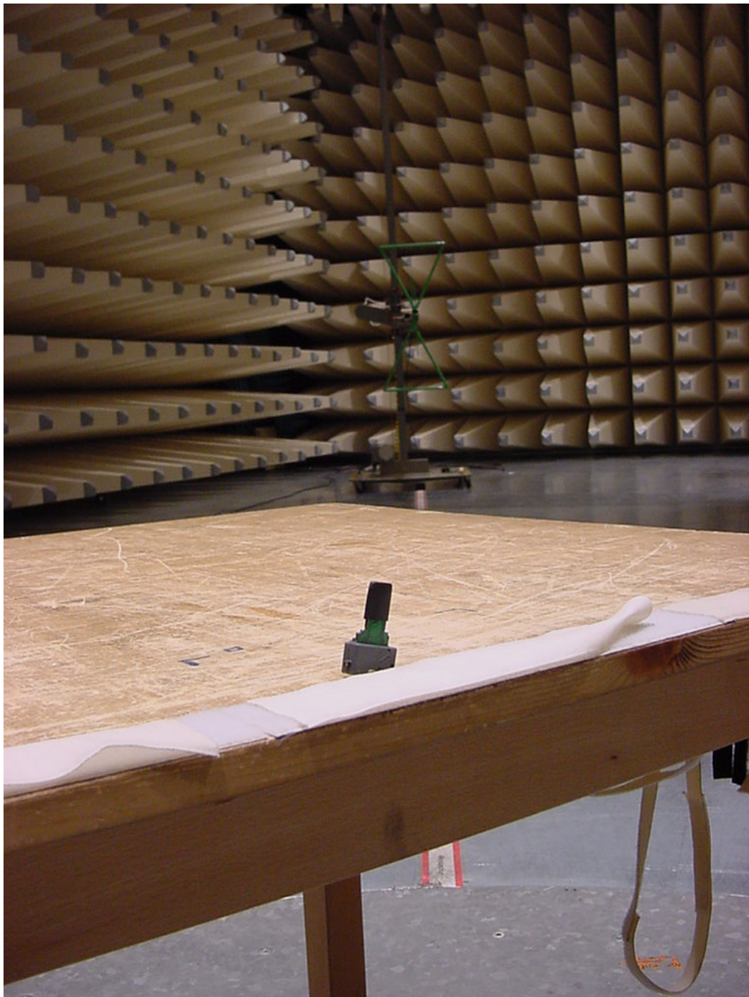
Photo 1 (Radiated Emissions): Tx with integrated antenna
