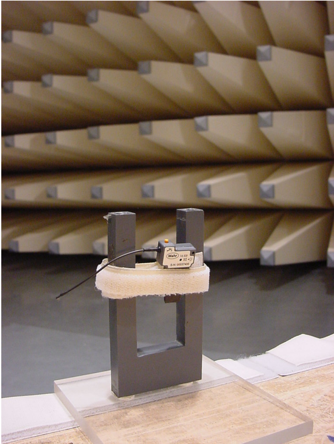
Photo 4 (Radiated Emissions): Tx with Lambda/8 antenna
