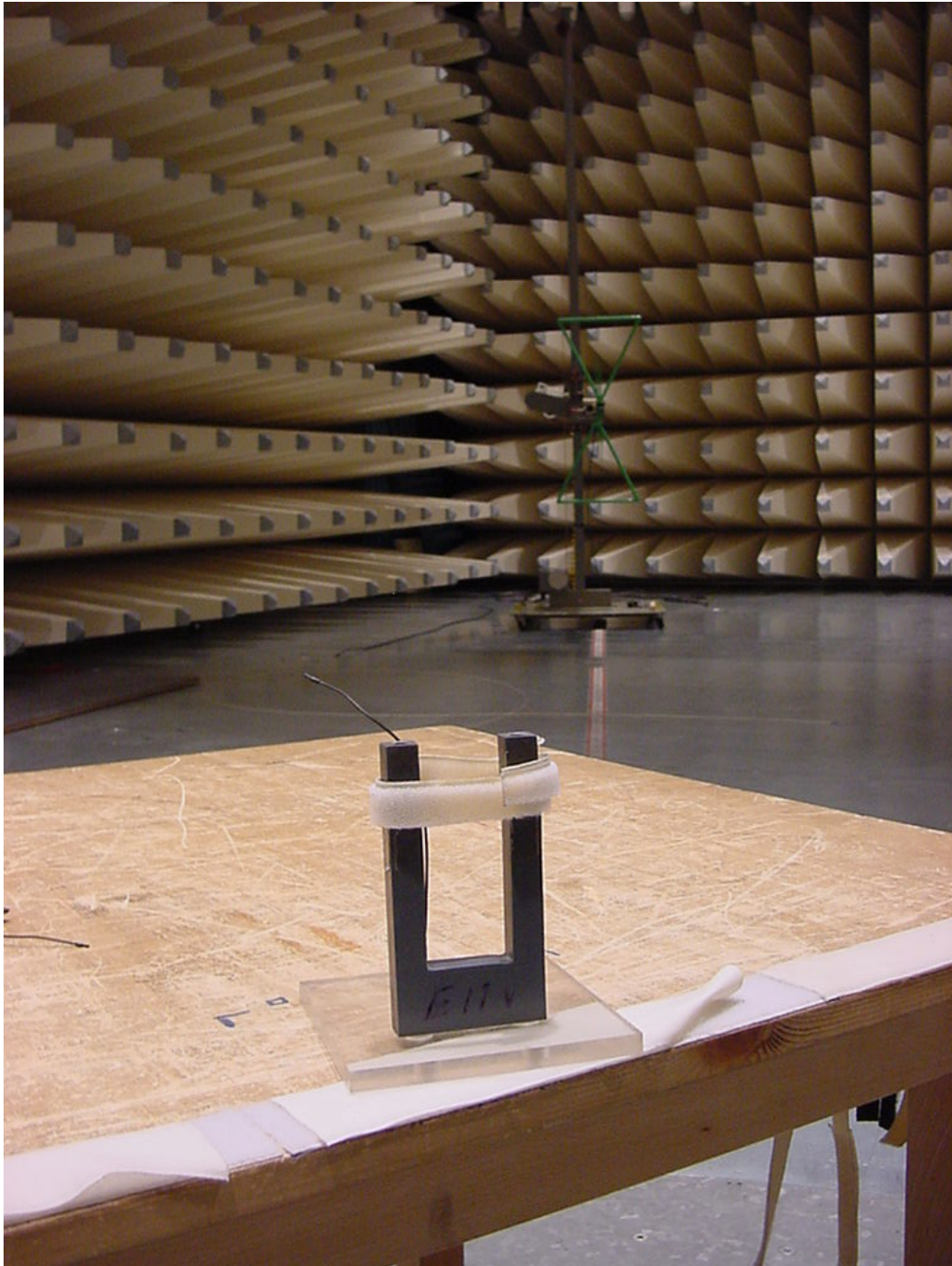
Photo 5 (Radiated Emissions): Tx with Lambda/4 antenna
