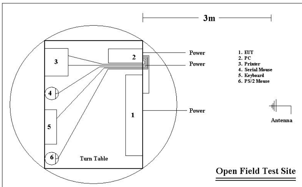
Radiated Emissions
