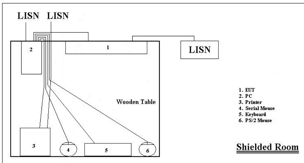
Conducted Emissions
