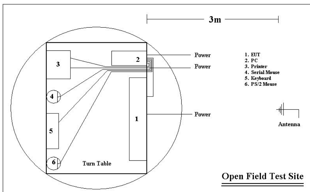
Radiated Emissions
