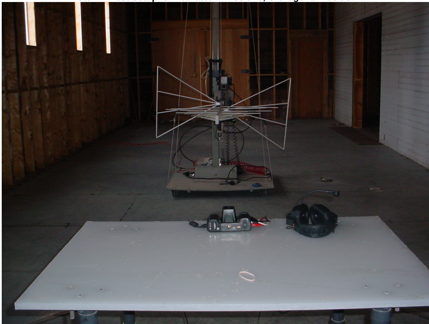
Photo #4: Test Setup for Radiated Emissions, Orthogonal Position #2
