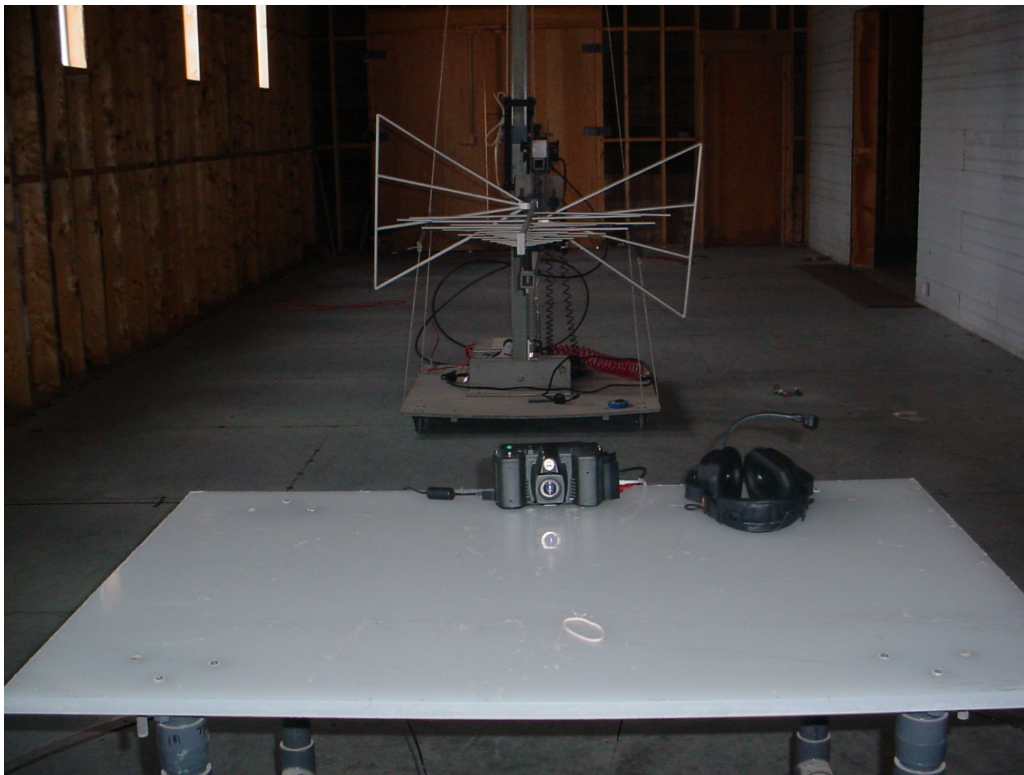
Photo #3: Test Setup for Radiated Emissions, Orthogonal Position #1
